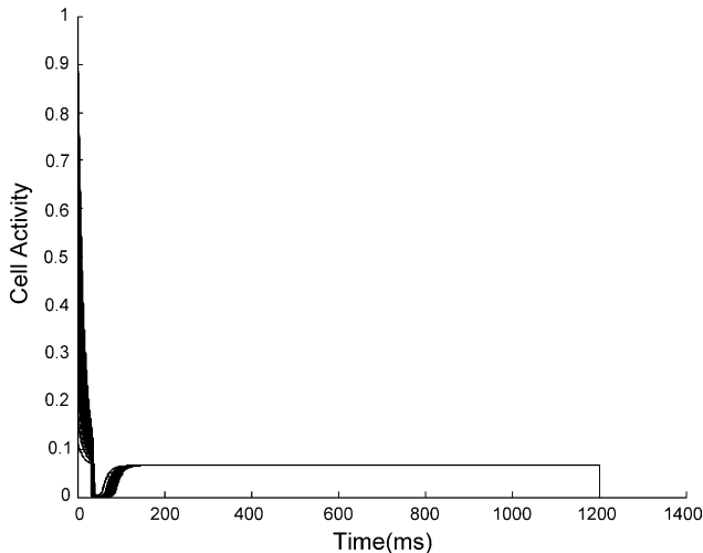
Fig. 4. This simulation shows that inputs within the on-center of the network from layer 6 to layer 4 can only provide excitatory modulation of layer 4 cells, but cannot fire these cells strongly. Strong inhibition within the off-surround can also occur.
