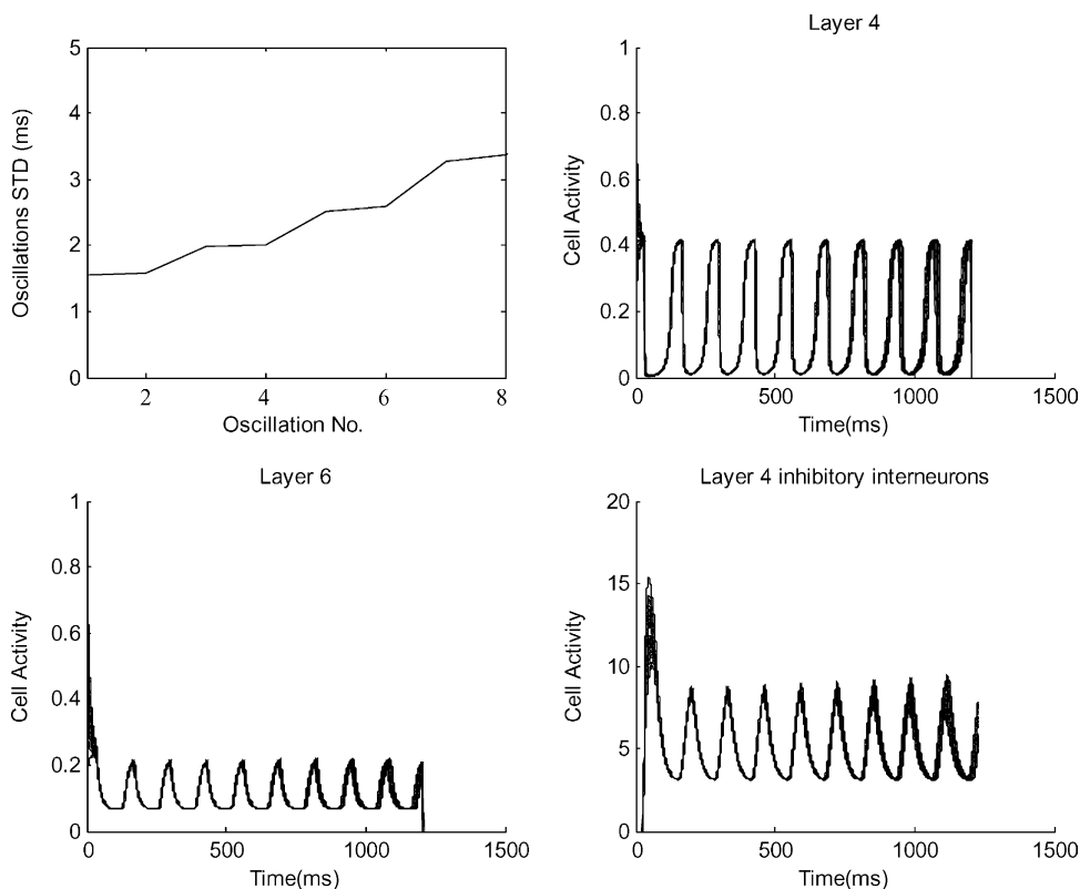
Fig. 3. Activity of the different layers of the LAMINART circuit with no horizontal bipole connections within layer 2/3. Each panel is composed of superimposed oscillatory activity of all 40 cells. Layer 4 excitatory, inhibitory, and layer 6 cell activities are shown. The initial activity of the all layer units are randomly set (uniform random distribution between 0.2 and 0.8) to bring them into different phase relations. This random initiation can be seen easily by looking at the ordinate of layer 6 and 4 activity panels. Fast resynchronization funnels all of the activities together within a small fraction of one oscillation period and afterward they oscillate together. The jitter curve shows that the jitter after this funneling-in of curves is on the order of 1–2 ms. There is also a slight increase of oscillation standard deviation in time (from \sim 1 to \sim 2 ms).
