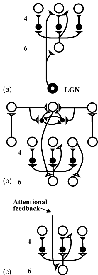
Fig. 2. Key circuit features of the LAMINART model: (a) LGN excites both layers 6 and 4. Layer 6 indirectly inhibits layer 4 through the inhibitory interneurons. Therefore, the excitation from layer 6 to layer 4 is modulatory (direct excitation approximately balanced by indirect inhibition). (b) Layer 4 directly excites layer 6. This combined with the 6→4 inhibition can generate oscillations in a suitable parameter range. Layer 4 also excites layer 2/3 cells, which have long horizontal axonal connections that also input to short-range inhibitory interneurons. The convergent excitation and inhibition results in the bipole property at target layer 2/3 cells. The cells in layer 2/3 send feedback to layer 6, which in turn subliminally excites layer 4 in the on-center and can strongly inhibit layer 4 cells through the off-surround. (c) Attention can also activate layer 6, and thereby have a modulatory effect on layer 4 that can help to select which grouping will win.
