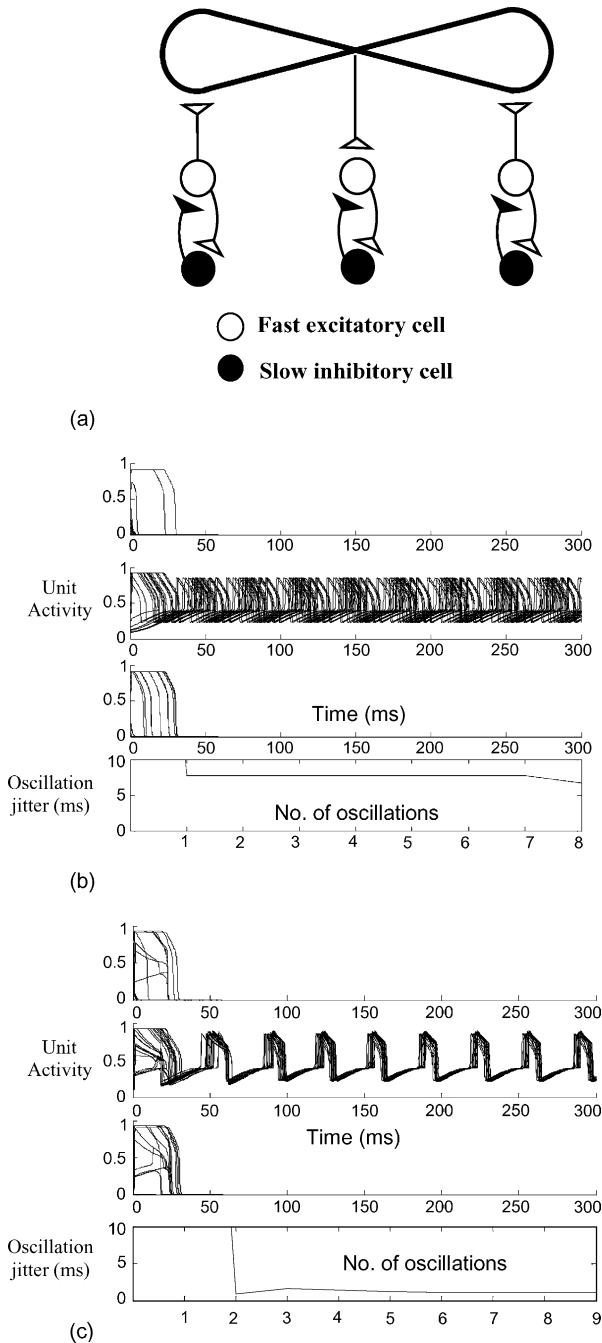
Fig. 1. (a) The architecture used by Grossberg and Somers (1991). Fast excitatory cells are connected to slow inhibitory cells. This fast versus slow time constant can generate oscillations in suitable situations. (b) If the cells are not connected, then their initial out-of-phase activities remain out-of-phase through time with an approximately constrain oscillation jitter. (c) The out-of-phase activities rapidly synchronize, within a single oscillation cycle.
