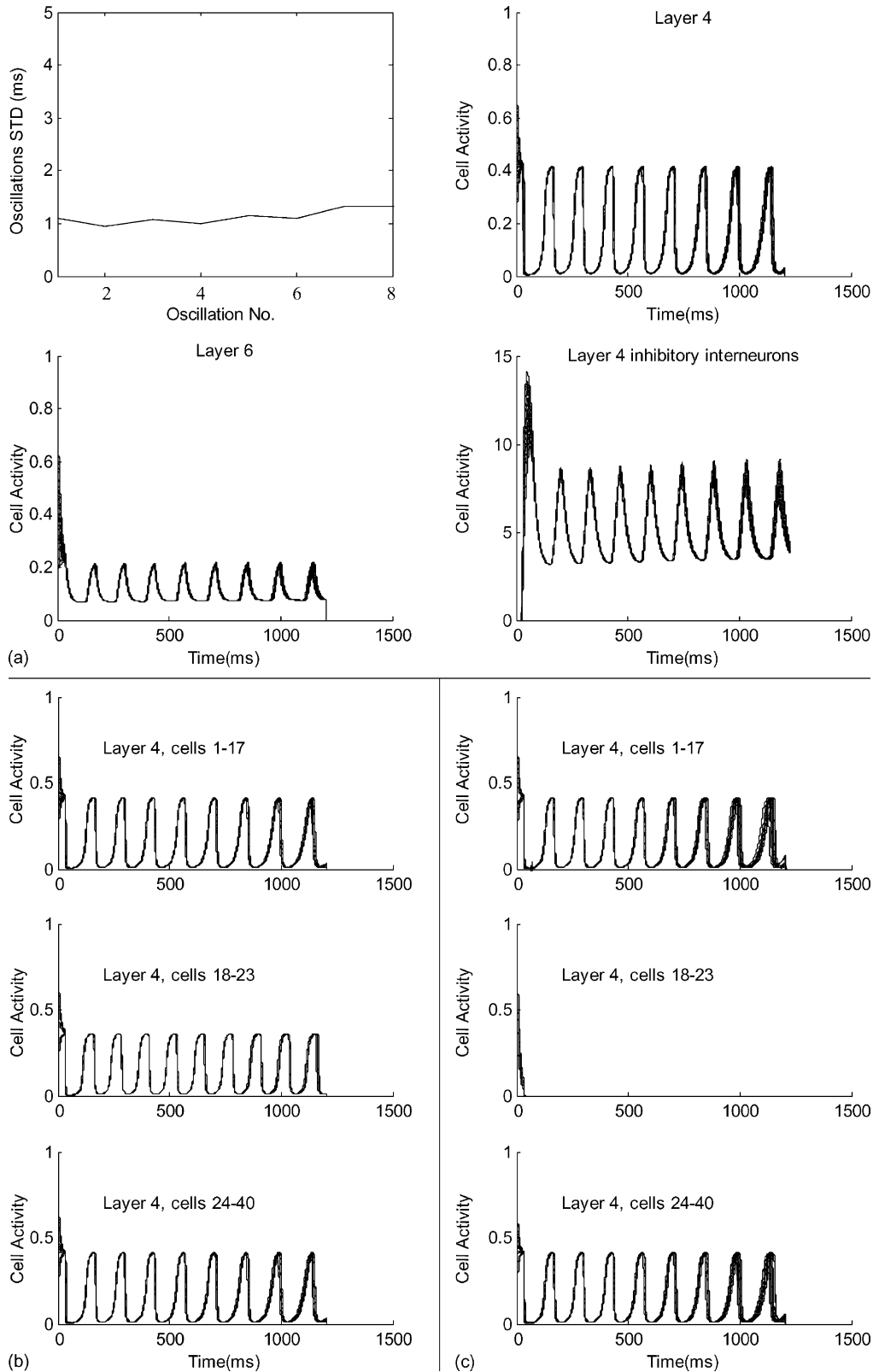
Fig. 6. Here, the bipole grouping cells are again included in (a) and (b), and constant inputs from the LGN are on. Again the network rapidly synchronizes, even though there are no LGN inputs to cells 18–23 of layers 6 and 4 in (b). Comparing the oscillation pattern with that in Fig. 3 shows that, first, the absolute value of the oscillation jitter is less and, second, that the slight increase of the oscillation jitter is less too. (c) When there is no bottom-up LGN input to cells 18–23, and no bipole grouping cells, then the initial randomized activities of these cells fade away. The lateral cells (1–17 and 24–40), however, follow the same pattern of fast synchronized oscillation as in (a) and (b). Thus, the bipole grouping cells are needed to complete groupings across occluded image regions to form illusory contours.
