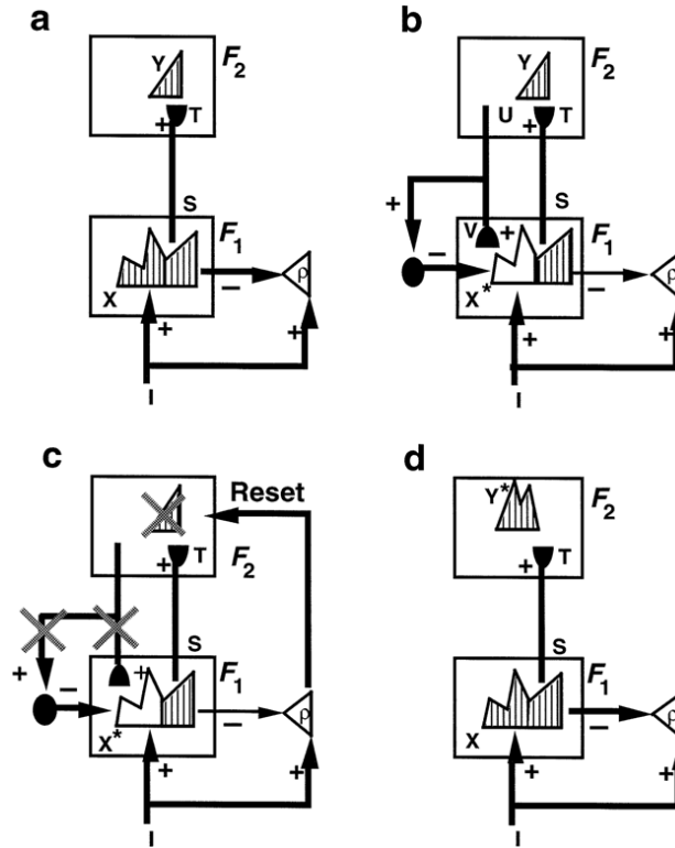
Figure 4 Search for a recognition code within an ART learning circuit: (a) The input pattern I is instated across the feature detectors at processing stage F_1 as a short term memory (STM) activity pattern X . Input I also nonspecifically activates the orienting system with a gain that is called vigilance ( \rho ); that is, all the input pathways converge with gain \rho onto the orienting system and try to activate it. STM pattern X is represented by the hatched pattern across F_1 . Pattern X both inhibits the orienting system and generates the output pattern S . Pattern S is multiplied by learned adaptive weights, also called long-term memory (LTM) traces. These LTM-gated signals are added at F_2 cells to form the input pattern T , which activates the STM pattern Y across the recognition categories coded at level F_2 . (b) Pattern Y generates the top-down output pattern U which is multiplied by top-down LTM traces and added at F_1 cells to form a prototype pattern V that encodes the learned expectation of the active F_2 nodes. Such a prototype represents the set of commonly shared features in all the input patterns capable of activating Y . If V mismatches I at F_1 , then a new STM activity pattern X^* is selected at F_1 . X^* is represented by the hatched pattern. It consists of the features of I that are confirmed by V . Mismatched
