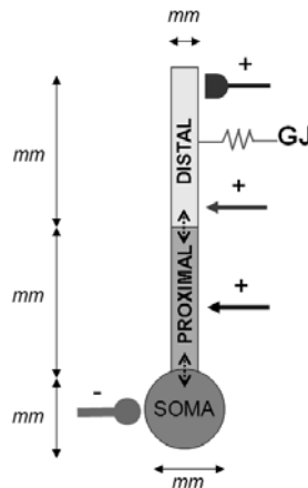
Figure 17 The generic neuron model. The neuron depicted above is a 3-compartment-cell with a soma, a proximal and a distal dendrite. Excitatory driving (arrow terminating in the proximal dendrite, +), modulatory (arrow terminating in the distal dendrite, +), plastic (half-ellipse terminating in the distal dendrite, +), as well as inhibitory (rounded arrow terminating in the soma, -) connections can terminate in each cell compartment,
