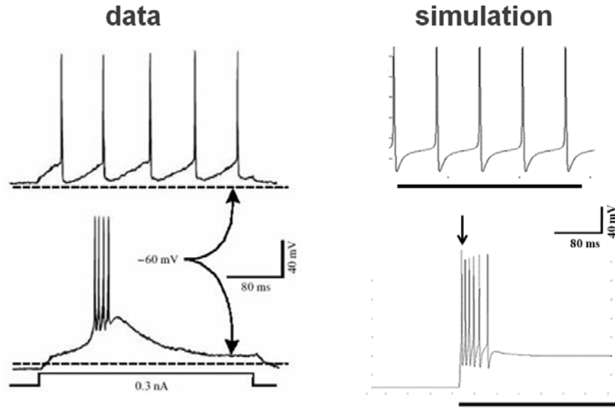
Figure 8 Burst and tonic firing in thalamic relay cells. Data : intracellularly in vitro recording illustrating the voltage dependency of the low threshold spike for a geniculate relay cell. The same depolarizing current pulse administered at two different initial holding potentials causes either tonic firing (top, cell depolarized, I_T inactivated) or burst firing (bottom, cell hyperpolarized, I_T de-inactivated). Modified and reprinted with permission from Sherman and Guillery, 2002. Simulation : a 0.3 nA current (horizontal bar) is injected in a simulated LGN cell in the absence (top) or presence (bottom) of a hyperpolarizing voltage clamp. The hyperpolarization of the cell and the presence of low-threshold Ca^{++} currents (see Equations (21)-(27) in Methods) causes the de-inactivation of the I_T current, inducing burst firing.
