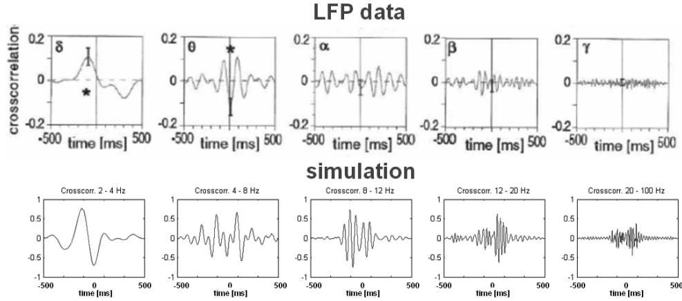
Figure 16 Data : Cross-correlation functions of local field potentials (LFP) from the middle layer of area 17 (primary visual cortical area) and lower layers of area 7 (higher-order visual area) during presentation of a no-go stimulus in behaving cats (reprinted with permission from Von Stein et al., 2000). Simulation : The activity of two thalamocortical loops was simulated, with a synaptic delay between layer 2/3 of the first-order cortical area and layer 4 of the second-order cortical area set at 10ms. Epochs of 1000ms were aligned to onset of a learned bottom-up stimulus that was presented for 1s prior to the beginning of the recording. Analysis was performed on a LFP recorder from two simulated 54-tip-electrodes from the two cortical areas, and data were separated in five different frequency ranges in accordance with classical electroencephalogram conventions: 2–4, 4–8, 8–12, 12–20, and 20–100Hz. The data were Fourier transformed and multiplied with the complex conjugate, and the inverse transformation was performed for selected frequency bins (corresponding to one “band”) to obtain cross-correlation functions for separate frequency ranges. Cross-correlation functions at different frequency bands was performed between LFP produced in the lower 0.3mm of the higher cortical area and the upper 0.3mm of the lower cortical area (both areas are 1.2mm thick).
