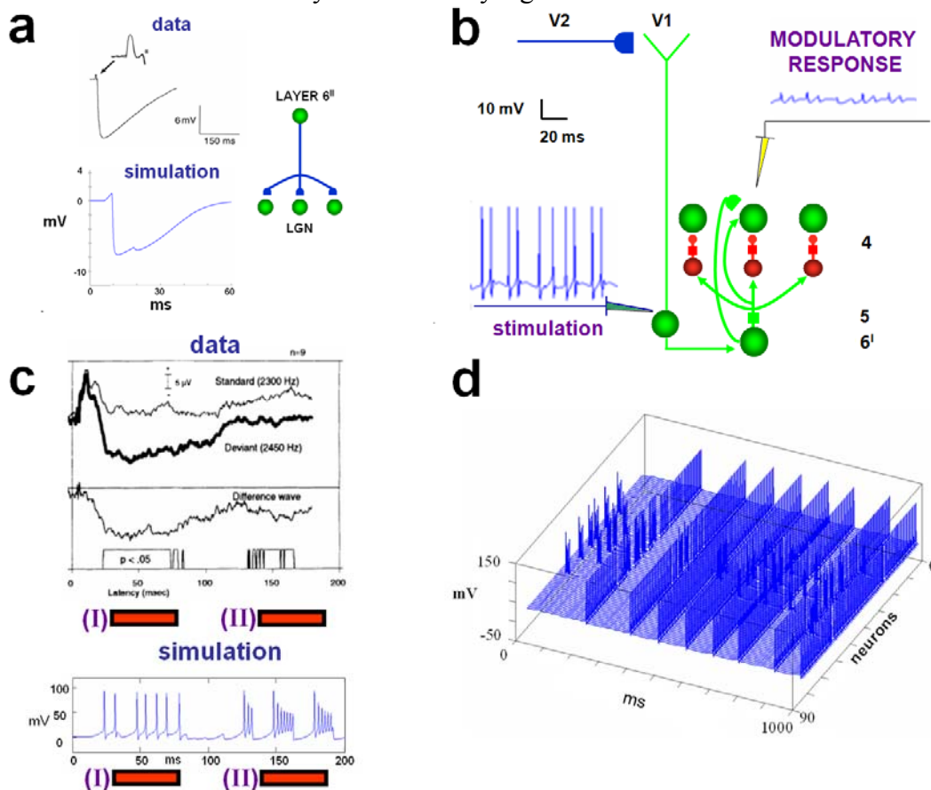
Figure 9 (a) Top-down corticothalamic feedback exerts a subthreshold excitatory effect on the membrane potential of thalamic relay cells. Data (upper left panel): whole-cell recording from a relay neuron in the somatosensory ventral posterior nucleus of a mouse thalamocortical slice in vitro . A single weak electrical stimulus (arrow) applied to a corticothalamic fiber elicits a small monosynaptic EPSP (asterisk in enlarged inset)
