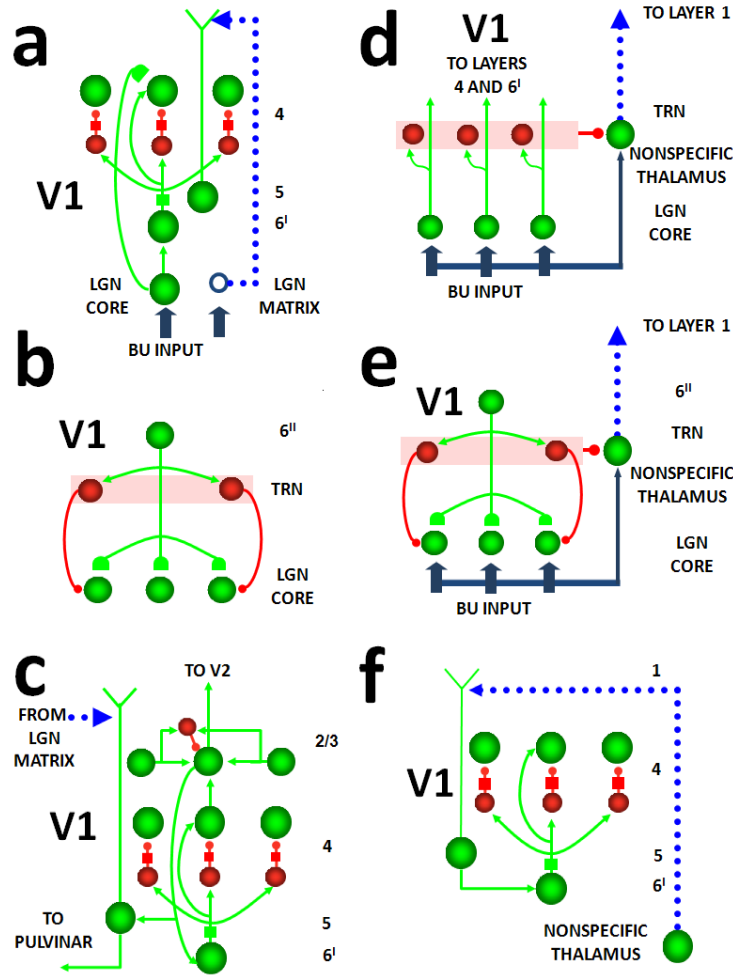
Figure 2 (a) LGN core cells in the specific pathway activate layer 4. LGN core cells also send axons to layer 6 I cells, and thereby also activate layer 4 via a 6 I →4 modulatory on-center, off-surround network that implements divisive contrast normalization of LGN inputs in layer 4. Layer 4 cells, in turn, activate cells in layer 2/3. In parallel, LGN matrix cell activation in the nonspecific pathway primes layer 5 cortical cells via excitatory connections to cortical layer 1, where layer 5 apical dendrites terminate. Layer 5 cells fire only when both matrix cells and layer 2/3 cells fire. Matrix cells hereby enable layer 5 cells to fire in response to layer 2/3 inputs, thereby closing the intracortical 4→2/3→5→6 I →4 resonant loop while activating driving inputs from layer 5 to the PULV. (b) Top-down feedback from V1 layer 6 II has a dual effect on LGN core cells: excitation via adaptive synapses (hemi-disks at ends of axonal pathways) and broad inhibition via the thalamic reticular nucleus (TRN) pathway. (c) Layer 2/3 cell outputs feed back to layer 5 cells, which can fire if matrix cells also input to the layer 1 apical dendrites of layer 5 cells. Layer 5 cell firing can, in turn, activate layer 6 I cells that activate layer 4 cells. Matrix cells hereby enable layer 5 cells to close the intracortical 4→2/3→5→6 I →4 resonant loop, even while they activate driving inputs from layer 5 to the PULV. (d) During bottom-up processing, bottom-up inputs send convergent excitatory signals to the nonspecific thalamus. In parallel, LGN core cells send specific inputs to layers 4 and 6 I of the cortex, as well as to TRN cells. The TRN cells, in turn, send convergent inhibition to the nonspecific thalamus. During bottom-up processing, the total excitatory and inhibitory signals are balanced, so that the nonspecific thalamus is not activated by the bottom-up input. (e) During top-down matching, layer 6 II cells excite TRN cells which, in turn, send inhibitory signals via a broad off-surround to LGN core cells. This inhibition helps to prevent cells that receive only bottom-up or top-down signals from firing, but not cells that receive both. Only LGN cells that receive matching bottom-up input and top-down cortical feedback cross the spiking threshold and propagate their activity to V1, while also (see
