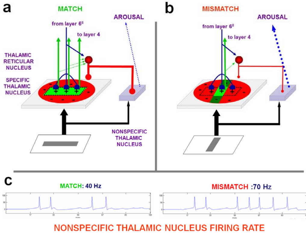
Figure 7 Regulation of nonspecific thalamic nucleus firing rate by the amount of match in the specific thalamic nucleus. (a) A bottom-up input pattern (horizontal bar, in green) is matched with a top-down expectation from layer 6 II (dotted horizontal bar) in the on-center (layer 6 II →specific thalamus) off-surround (layer 6 II →TRN→specific thalamus) corticothalamic loop. The convergent bottom-up excitation to the nonspecific thalamus is (partially or totally) cancelled by convergent TRN inhibition to the nonspecific thalamus. A spatial match (green horizontal area) allows specific thalamic cells to fire, excite their cortical target, and inhibit the nonspecific thalamus via the TRN. (b) A spatial mismatch between a bottom-up input pattern (vertical bar) and a top-down expectation (horizontal dotted bar) causes only a subset of specific thalamic cells to fire (bright green square area), excite their cortical target, and inhibit the nonspecific thalamus via the TRN. (c) Since the total, convergent bottom-up input to the nonspecific thalamus does not change in a match vs. a mismatch episode, the lower TRN firing rate during a mismatch triggers a higher firing rate in the nonspecific thalamus.
