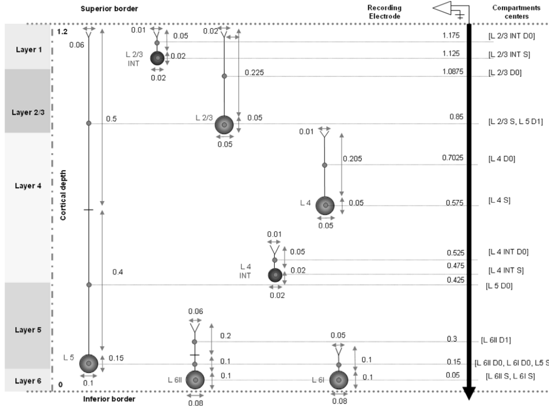
Figure 18 Spatial arrangement and cell sizes of the populations composing the 1.2mm thick laminar cortical sheet. A multi-compartment model with a spatially explicit structure allows to calculate transmembrane currents, which can be employed to derive aggregate cell recordings such as Local Field Potentials (LFP) and Current Source Densities (CSD). The activity of dendrites and cell somas of the populations can be recorded by an electrode with variable number of tips (black thick downward arrow, right). Since each compartment is treated as electrically uniform, the center of the compartment is the physical point at which the current source/sink is calculated (thick dot at the center of soma/dendrite). Cell bodies and dendrites are vertically aligned parallel to the recording electrode. For each layer, cells are displaced at random distance from the recording electrode. The distance of the electrode to the selected cell in the population is drawn from a uniform distribution on the interval [10 - 200] \mu m , whereas the distance to all other cells in the population is drawn from a uniform distribution on the interval [10 - 1000] \mu m . In the figure, only one cell for each population is shown. Abbreviations: L = layer; S = soma; D = dendrite (D0 = proximal dendrite; D1 = distal dendrite), INT = interneurons. All measurements are in mm.
