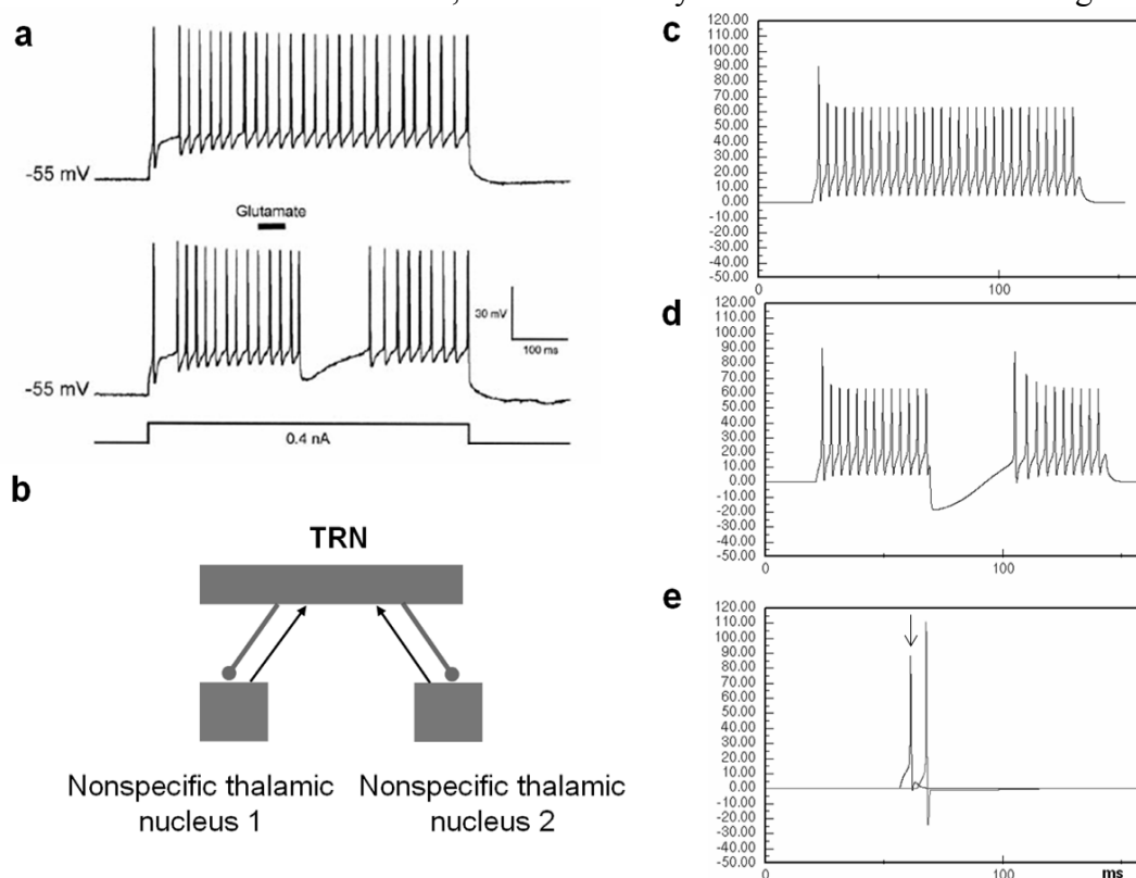
Figure 13 (a) Stimulation of one nonspecific thalamic nucleus interrupts a train of action potentials in another nonspecific thalamic nucleus. When held close to -55\text{mV} , a rostral intralaminar nucleus (RIL) cell responds with a train of action potentials (top recording) to a depolarizing 0.4\text{nA} current pulse (bottom, square wave). A train of action potentials (bottom recording) in the RIL cell in response to the depolarizing current pulse was interrupted by glutamate stimulation (black bar) in the caudal intralaminar nucleus (CIL, modified with permission from Crabtree and Isaac, 2002). (b) Model simulation includes two nonspecific thalamic nuclei and a
