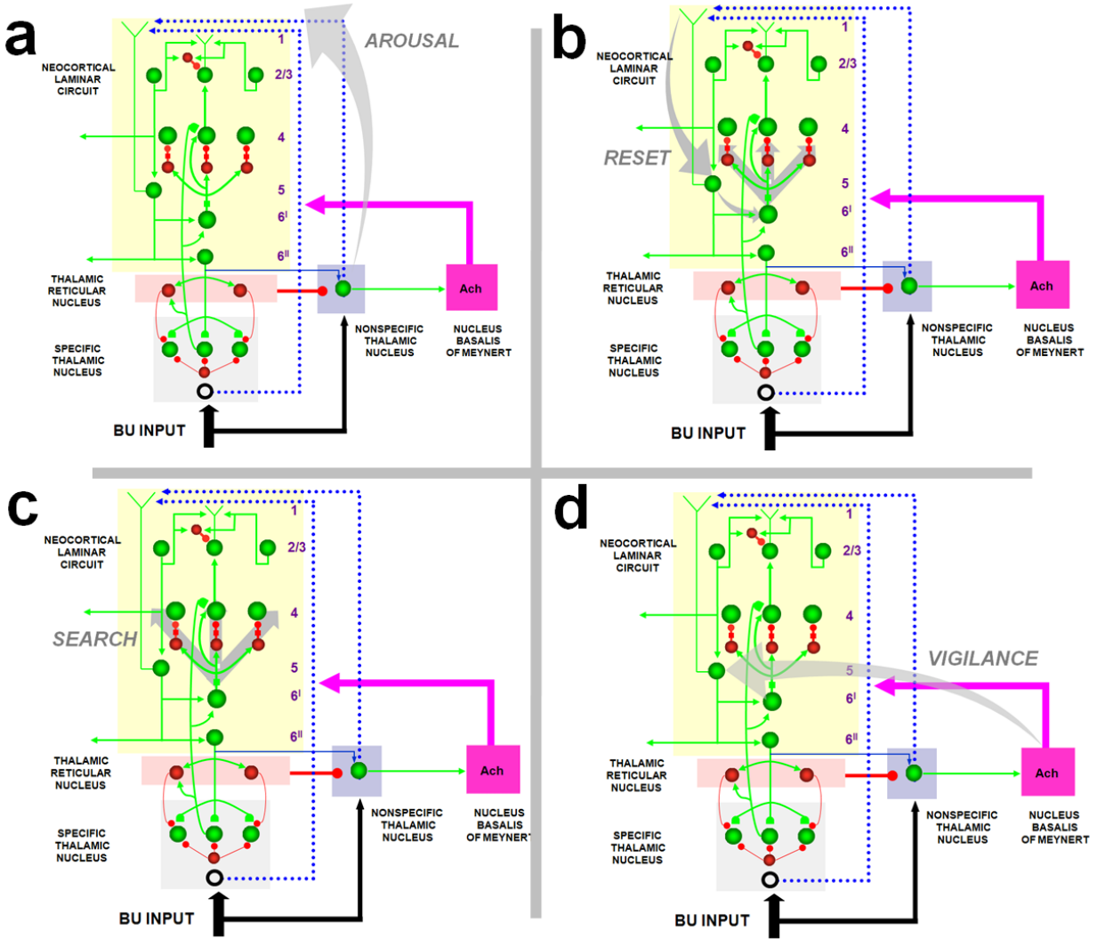
Figure 5 The large shaded gray arrows in the figure indicate the SMART pathways involved in the generation of the (a) AROUSAL burst, (b) RESET , (c) SEARCH , and (d), VIGILANCE control. See text for details.
