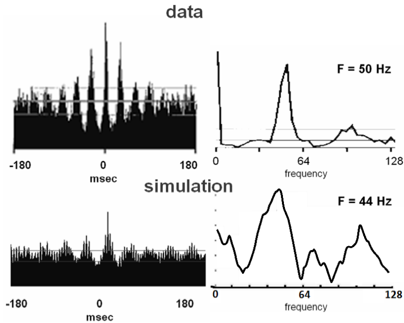
Figure 15 Example of short range ( 300\mu\text{m} ), single unit–single unit correlation of cells with overlapping receptive fields and similar orientation preference in V1; top, left : cross-correlation computed from the two spike trains during the response to the stimulus. top, right : power spectrum of the cross-correlation shown on the left, which shows a peak around 50Hz. Modified from Friedman-Hill et al. (2000). Bottom, left : cross-correlation computed from the spike trains of two nearby simulated layer 4 cells during stimulation of a learned stimulus (lines show the 95% confidence limit). Bottom, right : power spectrum of the cross-correlogram shown on the left.
