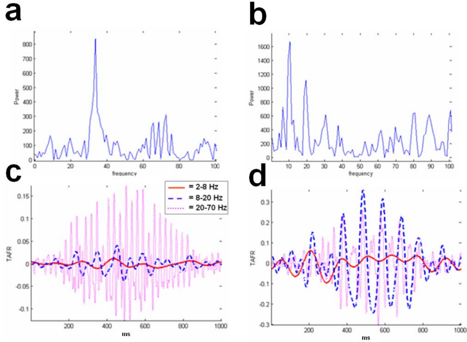
Figure 14 Power spectra of cumulative spike histograms of a laminar primary sensory cortical area during presentation of a stimulus (horizontal bar, 5 thalamic relay nuclei activated for 1000ms) during match (a) and mismatch (b) conditions show a peak in the slow \gamma frequency band (20-70Hz) in case of match, and lower frequencies in case of mismatch. The histograms were analyzed into three frequency bands ( \delta and \theta , 2–8Hz; \alpha and \beta , 8–20Hz; \gamma , 20–70Hz) to highlight the separate contribution of different oscillation frequencies in a match (c) and mismatch (d). Notably, \gamma oscillations are drastically reduced in a mismatch in favor of lower-frequency oscillations.
