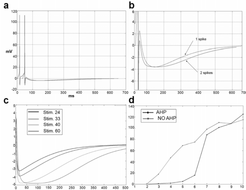
Figure 19 AHP-controlled inhibitory currents are spike-dependent. (a) Effect of cell spiking frequency on the membrane potential in the presence of AHP. The membrane potential of an isolated layer 5 pyramidal cell is plotted after emitting one (dotted trace) or two (continuous trace) spikes. Stimulation was induced by a 10ms current injection until one or two spikes were generated. In order to allow direct comparison of the membrane voltage, the second spike in the “two-spikes” condition and the only spike in the “one-spike” condition were aligned for comparison. (b) Magnification of (a) shows the different time course and amplitude of the membrane potential in the two conditions. (c) Higher firing rates, caused by higher currents injections of 24, 33, 40, and 60mV cause longer-lasting and deeper cell hyperpolarization, almost fully recovering after 500ms . (d) Firing rate
