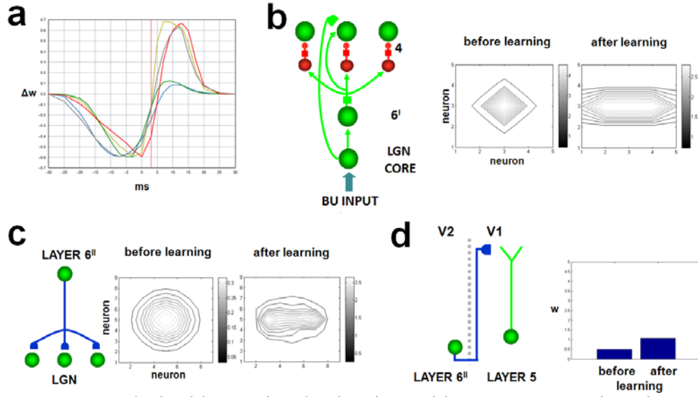
Figure 6 (a) STDP curves obtained by varying the time interval between presynaptic and postsynaptic spikes between [-30, 30] ms for five gating functions: grey (no gating), blue (dual OR gating), red (presynaptic gating), green (postsynaptic gating), yellow (dual AND gating), modified from Gorchetnikov et al. (2005b). (b) Presentation of a horizontal bar to a untrained thalamocortical circuit causes changes in the bottom-up synaptic weights of LGN→layer 4 synapses (postsynaptic gating, 100ms episode). (c) At the same time, TD layer 6 II →LGN weights change by adapting to the BU input shape (presynaptic gating). (d) Top-down synaptic weights at the connections from V2 layer 6 II to the layer 1 apical dendrites of layer 5 cells change during learning when layer 6 II feedback is active (dual AND gating). Episodes of asynchronous activities can occur at learnable synaptic stages in different cortical areas. Dual AND gating prevents learning when only V2 layer 6 II cells are active and no activity is present in V1 layer 5.
