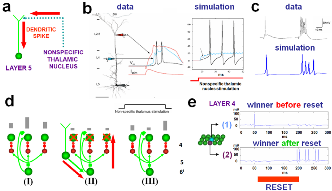
Figure 10 (a) In the model, an increase in nonspecific thalamic firing rate during a mismatch nonspecifically activates layer 1, including apical dendrites of layer 5 cells, where dendritic spikes are triggered that can cause
