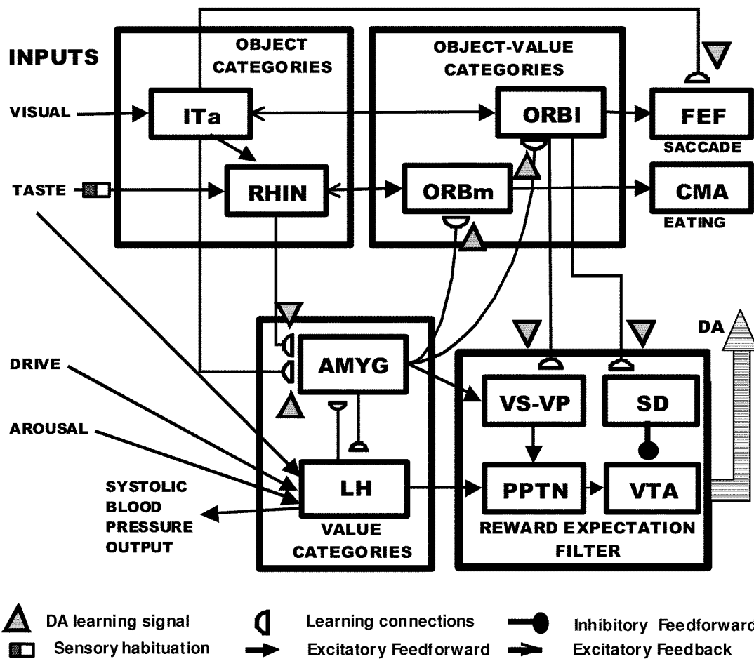
Figure 1: MOTIVATOR model circuitry. The model receives four types of inputs: visual, gustatory, drive (metabolite-related signals), and arousal. The model generates
