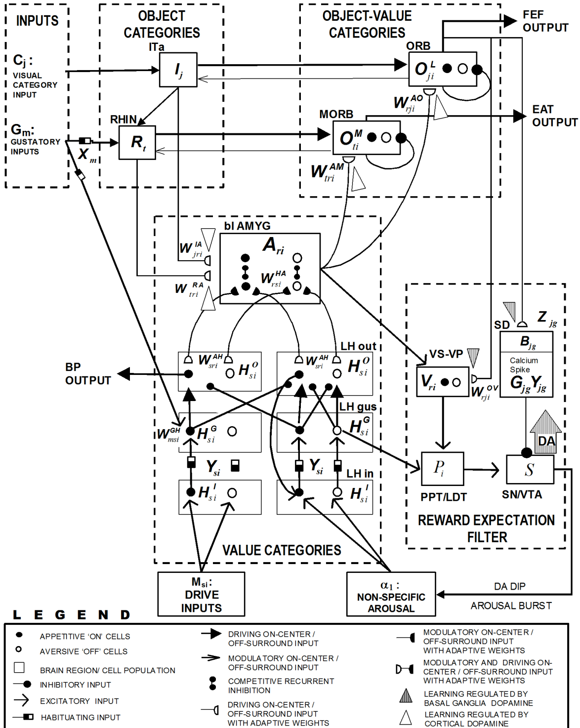
Figure 5: Model detail with equation variables. Distinct cell types are represented with different labeled compartments. Cells may or may not show a selective response to affective information of different valences. Cells which selectively respond to appetitively valenced information are indicated by filled circles. Cells which selectively
