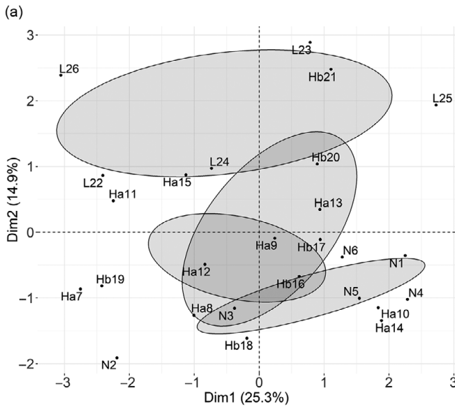
Figure 10.6 Representations of individuals according to Mandarin phonetic variables in MFA3. (a) Representations of individuals in terms of summed projections of all the variables in their Mandarin phonetic profile on Dim1 and Dim2 in MFA3 (ellipses mark the 95% CI around group means); (b) Mandarin phonetic profiles of four peripheral individuals (N5, L23, Ha12, Hb20) in terms of the six variable groups.
