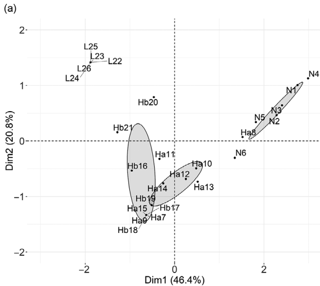
Figure 10.2 Representations of individuals according to demographic variables in MFA1. (a) Representations of individuals in terms of summed projections of all the variables in their demographic profile on Dim1 and Dim2 in MFA1 (ellipses mark the 95% CI around group means); (b) Demographic profiles of three peripheral individuals (N4, L25, Ha9) in terms of the three variable groups.
