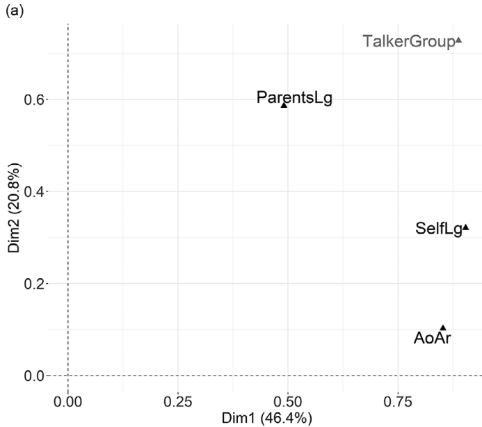
Figure 10.1 Variable groups and categorical variables (by level) in MFA1. (a) Representations of variable groups, including latent TalkerGroup , in terms of the first two dimensions (Dim1, Dim2) of MFA1 over the whole participant sample; (b) Mean representations of each level of the categorical variables (prefixes indicate variable group; Self = SelfLg , Prnt = ParentsLg ).
