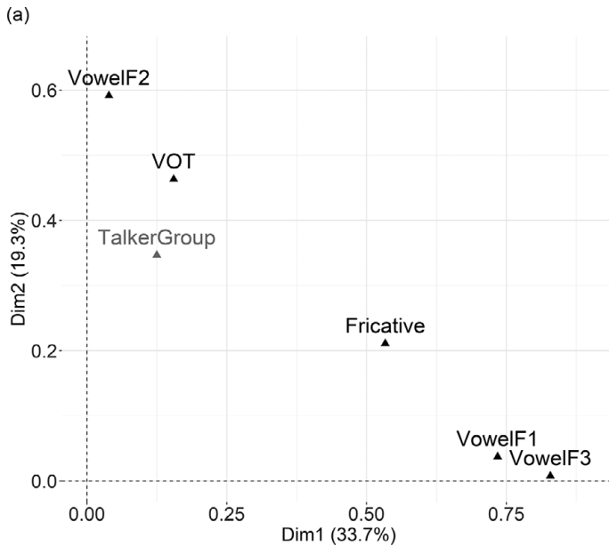
Figure 10.8 Variable groups and English phonetic variables in MFA4. (a) Representations of variable groups, including latent TalkerGroup , in terms of the first two dimensions (Dim1, Dim2) of MFA4; (b) Mean representations of phonetic variables (prefixes indicate variable group; F1 = VowelF1 , F2 = VowelF2 , F3 = VowelF3 , Fric = Fricative ).
