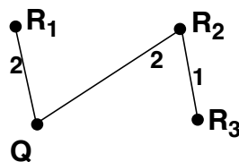
Figure 2: KMB algorithm.
