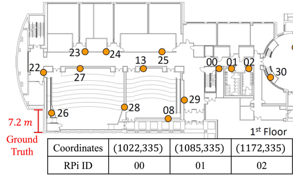
Fig. 9. Coordinates of the RPi and the ground truth of distance.
