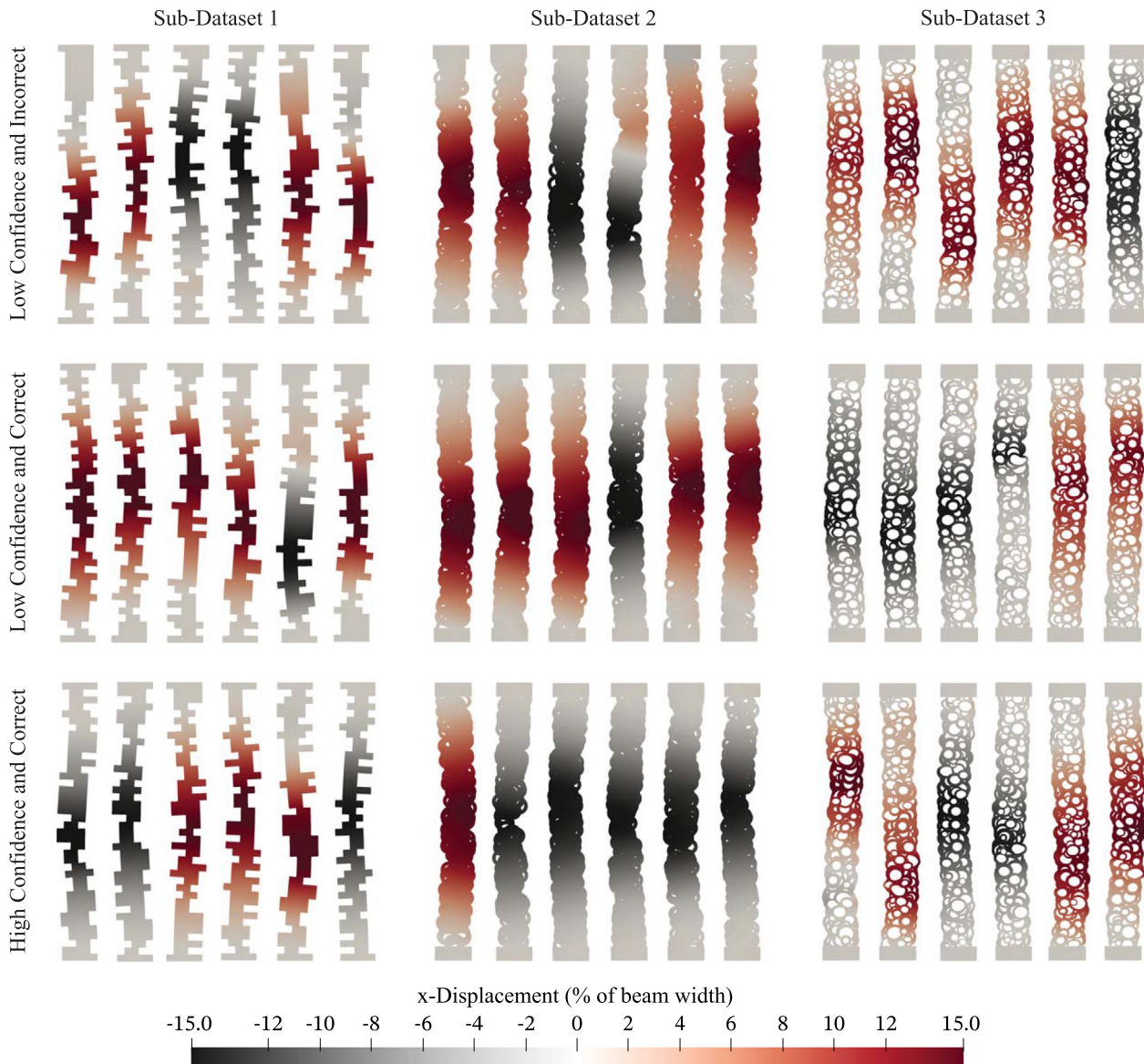
Fig. 13. Examples of deformed columns for high and low confidence predictions. Structures are arranged according to confidence levels (with low being 50% probability of being in either class and high being 100% in the correct class) and accuracy of prediction.
