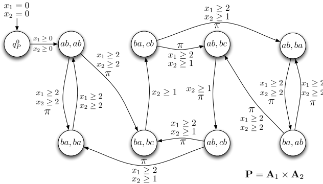
Fig. 3: The product timed automaton \mathbf{P} describing the motion of the two robots. The state ab, ba denotes that \mathbf{A}_1 is in state ab and \mathbf{A}_2 is in state ba . To avoid notation clustering, we do not show the clock-resets and invalid transitions. For example, in the transition from state (ba, bc) to (ba, cb) , robot 2 completes a transition, so its clock is reset, while robot 1 does not complete a transition, the state stays the same and the clock is not reset. The transition from (ba, bc) to (ab, bc) is invalid, because it can never happen before the transition from (ba, bc) to (ba, cb) .
