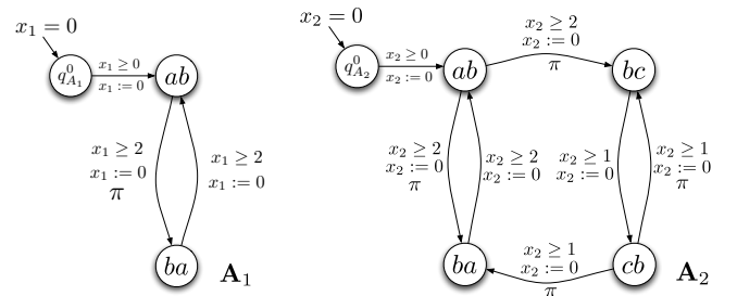
Fig. 2: Timed automata \mathbf{A}_1 and \mathbf{A}_2 of each robot, corresponding to \mathbf{D}_1 and \mathbf{D}_2 shown in Fig. 1c and Fig. 1d, respectively. The equations next to each arrow represents the clock constraint and the clock-reset associated with each transition of the timed automaton.
