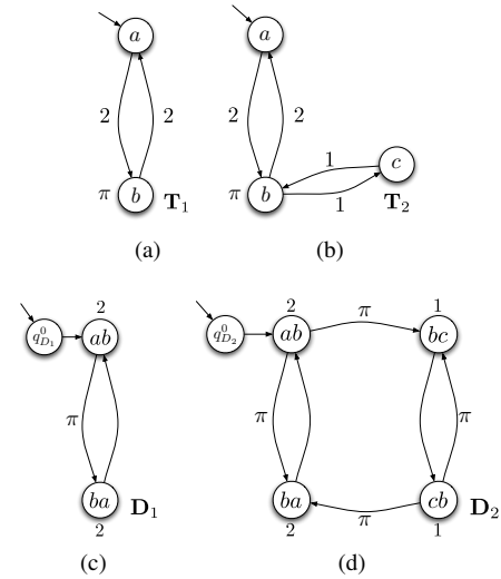
Fig. 1: (a) and (b) show the transition systems \mathbf{T}_1 and \mathbf{T}_2 for two robots in an environment with three vertices. The states of the transition systems correspond to vertices \{a, b, c\} and the edges represent the motion capabilities of each robot. The weights of the edges represent the time needed to traverse from a state to another; (c) and (d) are the dual transition systems \mathbf{D}_1 and \mathbf{D}_2 corresponding to \mathbf{T}_1 and \mathbf{T}_2 , respectively. A state labelled ab means that the robot is travelling from vertex a to b .
