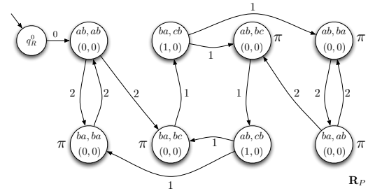
Fig. 4: The finite state region automaton capturing the joint behavior of two robots in 9 states. In the circle representing a state \{q, r\} , the first line is q and the second line is r .
