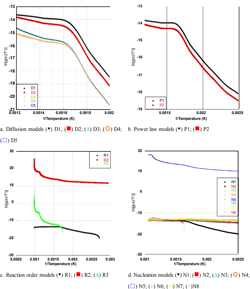
Figure 5: Non-isothermal decomposition of FC at 100K/min fit to various models according to Table 2
