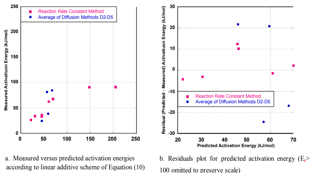
Figure 8: Applicability of linear addition scheme to predict activation energies of FC:IL blends using (■) R1 and (•) average of D2-D5
