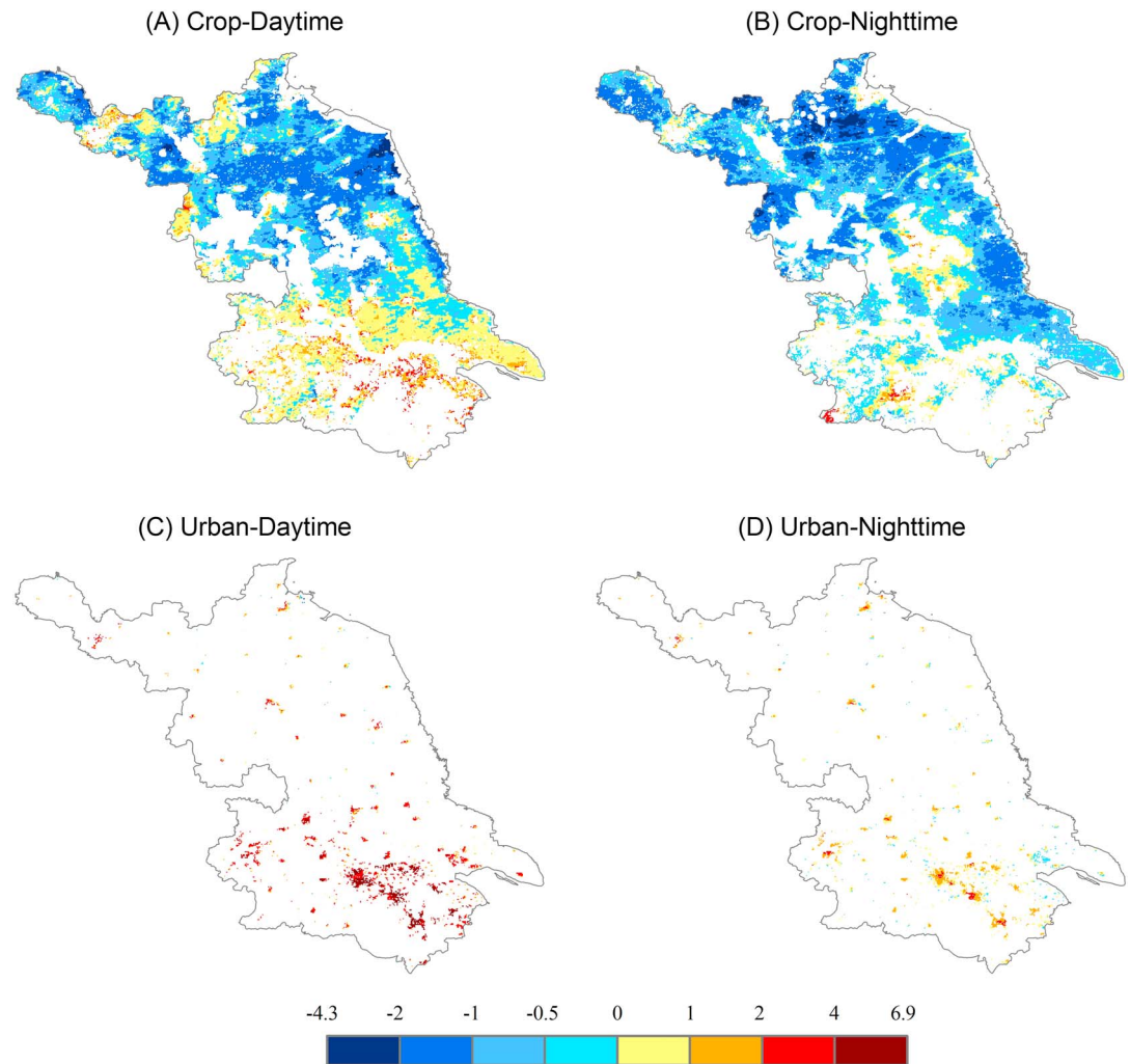
Figure 3. Spatial distributions of the annual mean \Delta T (°C) for (a, b) crop and (c, d) urban lands in Jiangsu Province, eastern China. The \Delta T of mixed lands were not shown.
