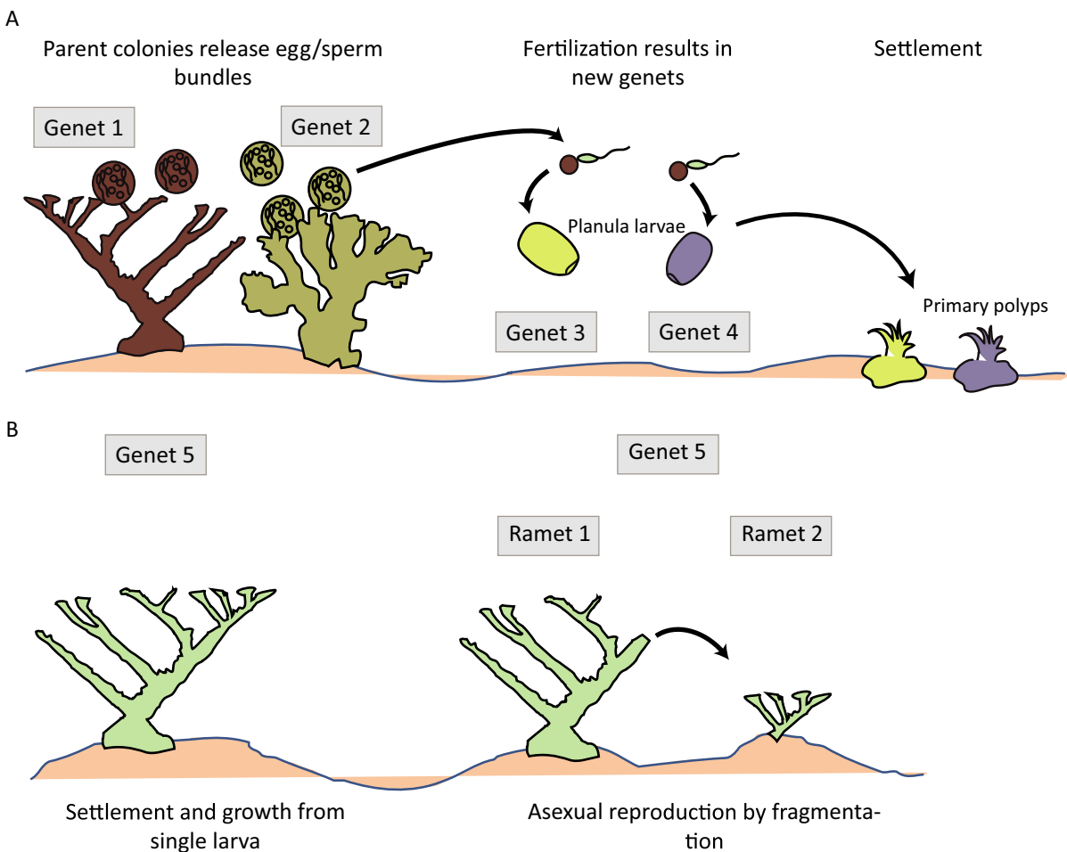
FIG 2. Coral reproduction. (A) Most reef-building species in the Caribbean are self-incompatible hermaphroditic broadcast spawners. Adult colonies release egg–sperm bundles that float to the surface where they break apart and mix with gametes from other colonies of the same species. After fertilization and development, larvae settle onto the reef, metamorphose into primary polyps, and grow into new genets. (B) Over time, genets may fragment. These fragments can reattach to form new ramets of the same genet. A genet is defined as a genetically unique colony or collection of colonies (ramets) that can trace their ancestry back to the same sexual reproductive event (i.e., they stem from the same settler and, hence, share the same genome). Adopted from Devlin-Durante et al. (2016).
