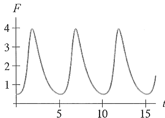
Figure 2.2 The F(t) -graph if R_0 = 1 and F_0 = 0.5 .
