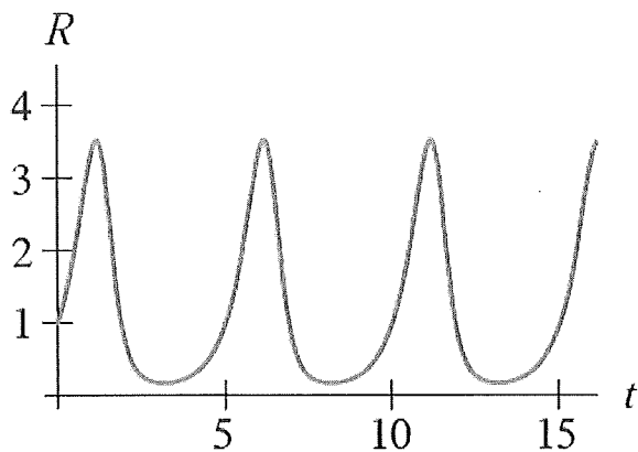
Figure 2.1 The R(t) -graph if R_0 = 1 and F_0 = 0.5 .
