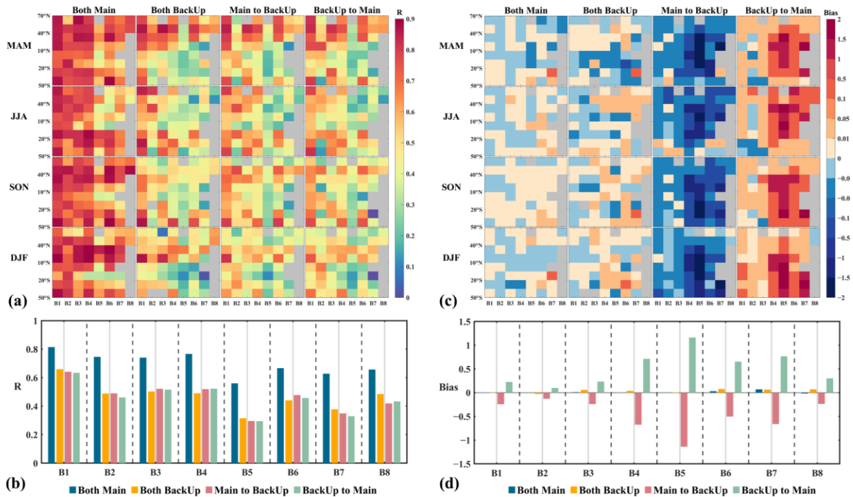
Fig. 8. (a) Heat map of R between pixel pairs for two adjacent years. (b) Mean values of R for LAI pixel pairs for all latitudinal bands and seasons across eight biome types. (c) Heat map of Bias between pixel pairs for two adjacent years. (d) Mean values of Bias for LAI pixel pairs for all latitudinal bands and seasons across eight biome types. Obtained by averaging three sets of results for 2003-2004, 2010-2011, and 2020-2021. Each grid cell represents all pixels of a particular biome type within the 15° latitude band. Only pixels with no change in vegetation type between adjacent years were used as analyzed pixels. Grey cells indicate a lack of vegetation pixels or fewer than 50 valid pixels.
