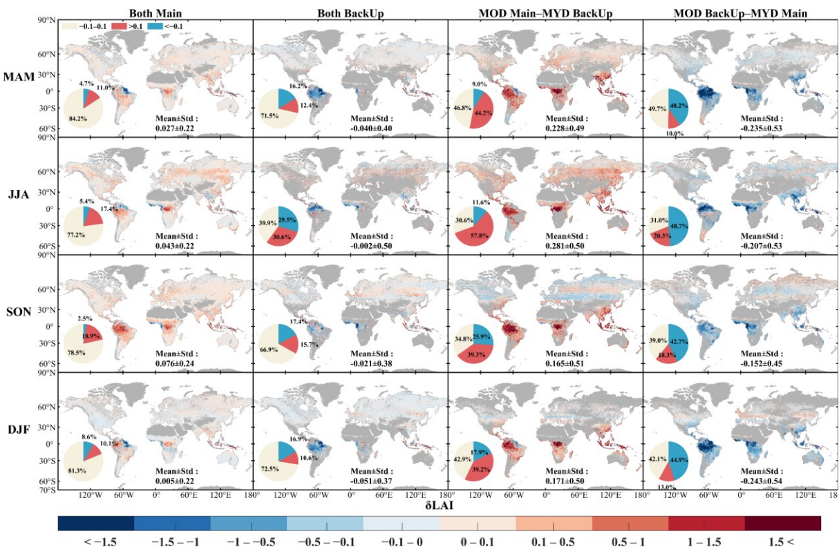
Fig. 5. Global distribution of LAI differences (MOD15A2H–MYD1512H) for different combinations of Terra and Aqua algorithms for the period 2003 to 2021. Results are from seasonal means and multi-year means of each composite difference.
