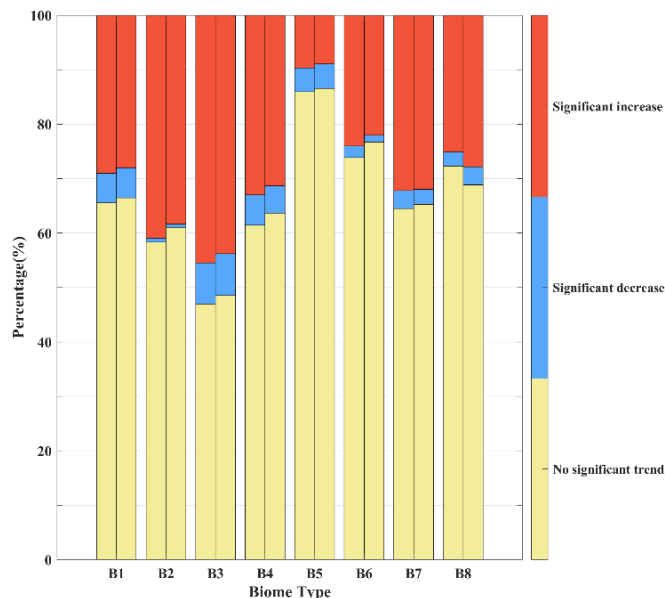
Fig. 12. Percentage of trends in Main LAI (left bars) and Mixed LAI (right bars) by biome type. The trend was categorized as no significant trend if it did not pass the significance test or passed the significance test but the absolute value of the change was less than 0.001 and as a significant increase (decrease) if it passed the significance test and the absolute value of the change was greater than 0.001. Only pixels with no change in land cover between 2002 and 2021 were used as analyzed pixels.
