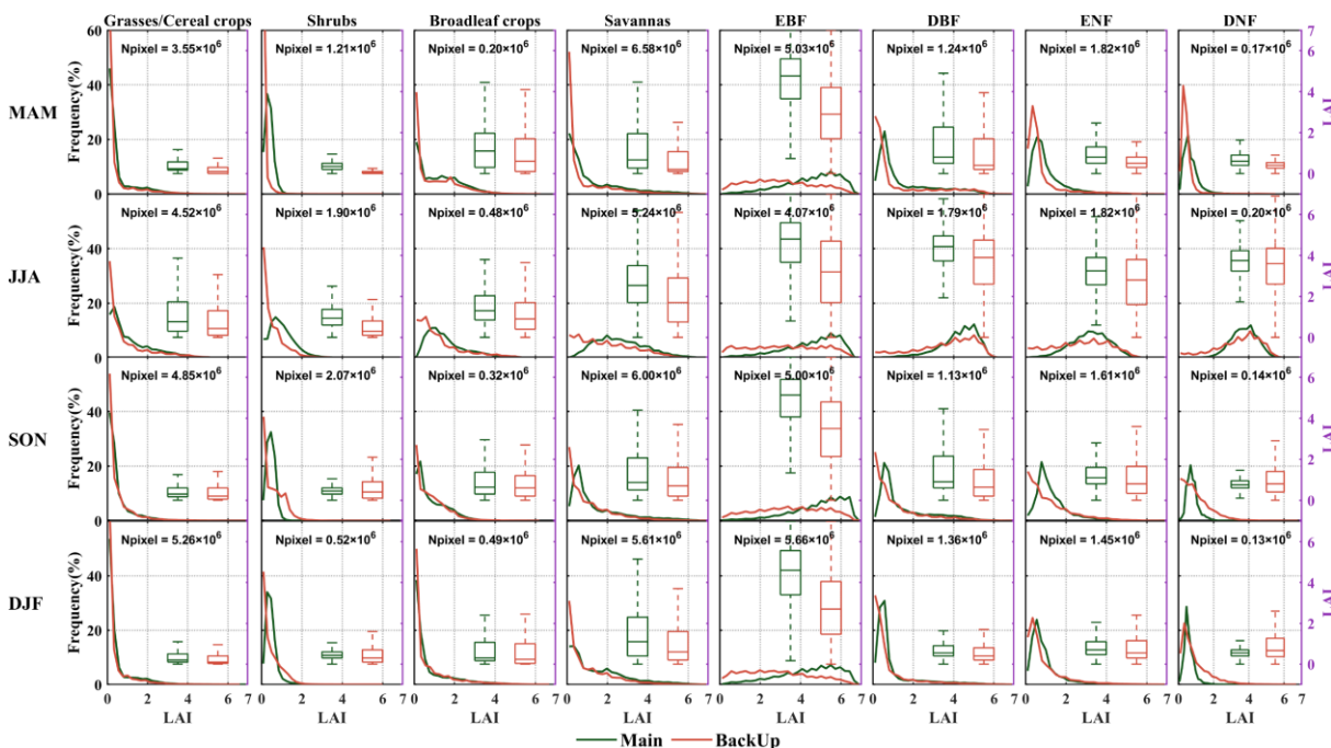
Fig. 4. Histogram and box plots of monthly average LAI for the main and backup algorithms for the period 2017–2021, including median, quartiles and whiskers. Only pixels with both main and backup algorithms in one month were used as analysis pixels. Bin in the frequency distribution histogram is 30. The first y-axis (left) represents the y-axis of the histogram of the frequency distribution and the second y-axis (right) represents the y-axis of the box plots. Only pixels with no change in land cover between 2017 and 2021 were used as analyzed pixels.
