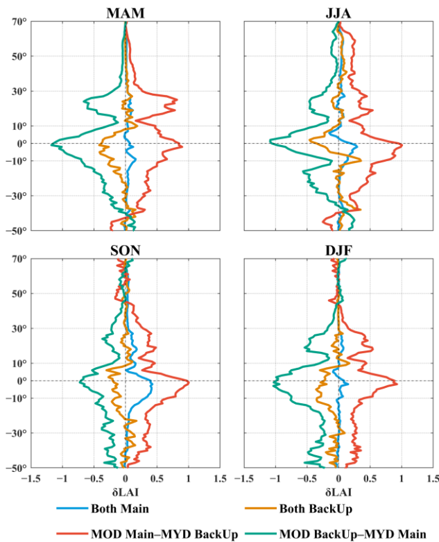
Fig. 6. Distribution of latitudinal mean differences for different algorithm LAI of MOD15A2H and MYD15A2H. The latitude interval is 1°.
