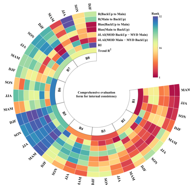
Fig. 13. The internal consistency of the eight biome types is comprehensively ranked based on the above findings. A smaller Rank indicates higher consistency or quality according to this index. Where Trend R^2 represents the trend consistency of Main LAI and Mixed LAI (growing season only); RI represents the proportion of main algorithm retrievals in 2021; \delta LAI indicates the difference in retrievals by different algorithms for Terra and Aqua, while R and Bias represent the correlation and bias of pixels in adjacent years.
