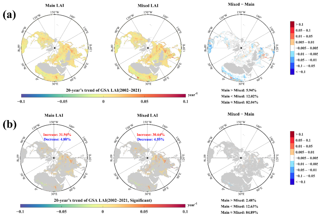
Fig. 10. Spatial distribution of GSA LAI trends and their differences under different algorithm control methods. (a) The trend estimates were based on Sen's slopes. (b) The trend estimates that passes the MK significance test ( P < 0.1 ). The white areas on the surface are considered to be roughly equal when the differences are small.
