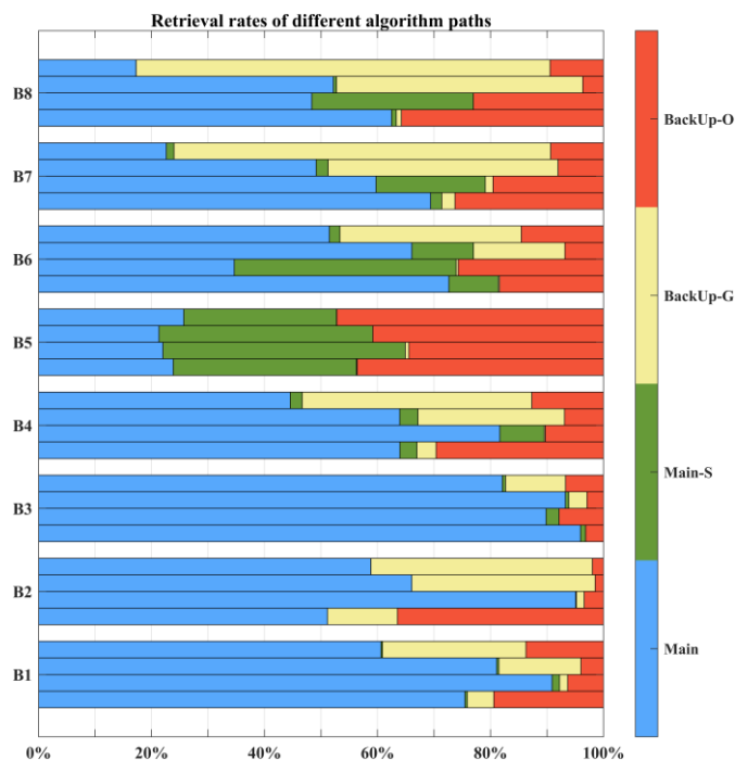
Fig. 3. Retrieval rates of different algorithm paths for different biome types globally. Comparisons are made for the four periods MAM, JJA, SON, and DJF (four bars from bottom to top).
