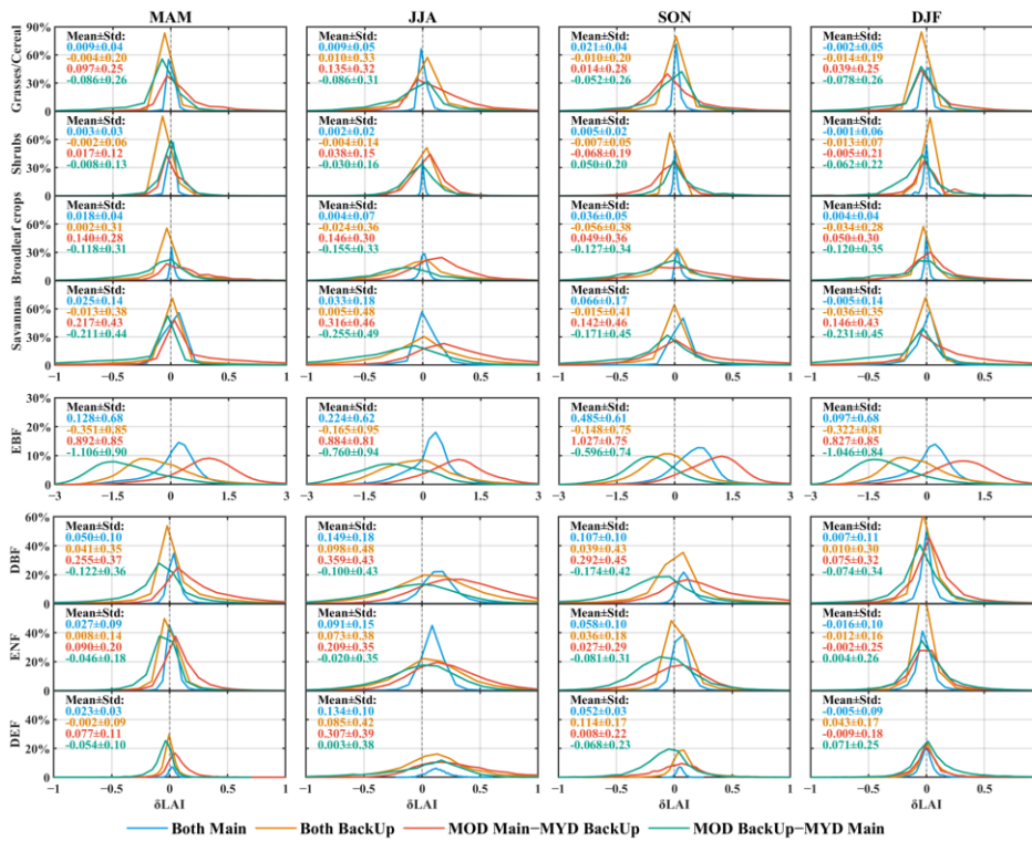
Fig. 7. The frequency histogram curves of LAI differences for different algorithm paths. These curves were generated from the data in Statistical Fig. 5, and the analysis only included pixels where the biome type did not change over the 19 years. The bin size is set to 70.
