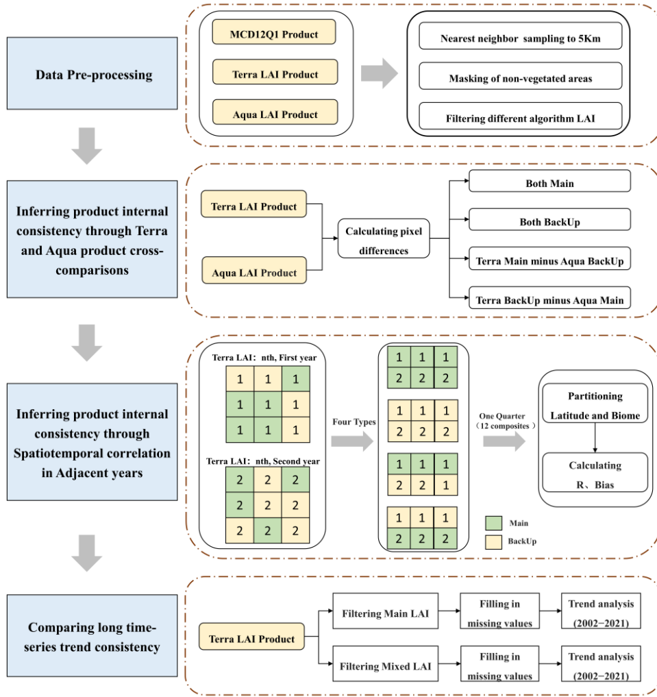
Fig. 1. The framework of internal consistency evaluation.
