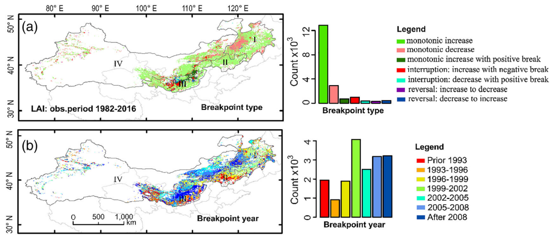
FIGURE 2 Spatial distribution of per-pixel leaf area index (LAI) breakpoints detected by Breaks for Additive Season and Trend (BFAT). (a) Spatial distribution of seven breakpoint classes. (b) Spatial distribution of the year of breakpoint detection [Colour figure can be viewed at wileyonlinelibrary.com ]
