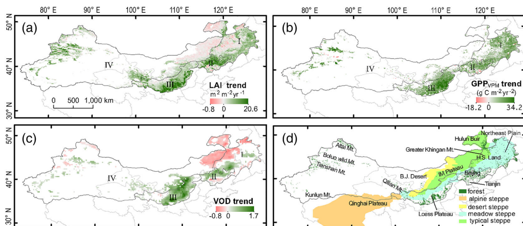
FIGURE 5 Vegetation trends and vegetation types in the study area. (a) Leaf area index (LAI) trends ( p value < .05 , n = 35 ) from 1982 to 2016. (b) GPP VPM trends ( p value < .05 , n = 17 ) from 2000 to 2016. (c) Vegetation optical depth (VOD) trends ( p value < 0.05 , n = 21 ) from 1992 to 2012. (d) Vegetation types. White areas (Figure a–c) represent the slope is close to zero or bare ground [Colour figure can be viewed at wileyonlinelibrary.com ]
