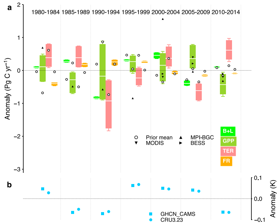
Figure 3. Detrended anomalies of (a) carbon fluxes and (b) temperature. The whisker-box plot indicates the range, interquartile, and mean of posterior values from the nine tests. Different markers represent prior mean values from TRENDY models and observation-based GPP values. Note that fluxes to the atmosphere are defined as positive, which means a negative anomaly of GPP or B + L indicating an increase of GPP and land sink while a negative anomaly of TER and FR indicating a decrease of TER and FR.
