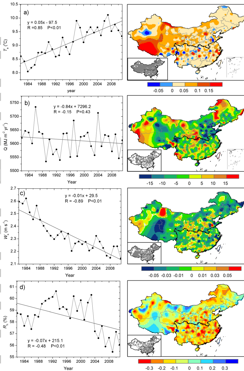
Figure 9. Time series (left) of annual (a) average T_a , (b) surface solar radiation Q , (c) average W_s , and (d) average R_h and (right) their linear trends and significance ( P < 0.05 shown in grey color in the hatch) in China during 1982-2011.
