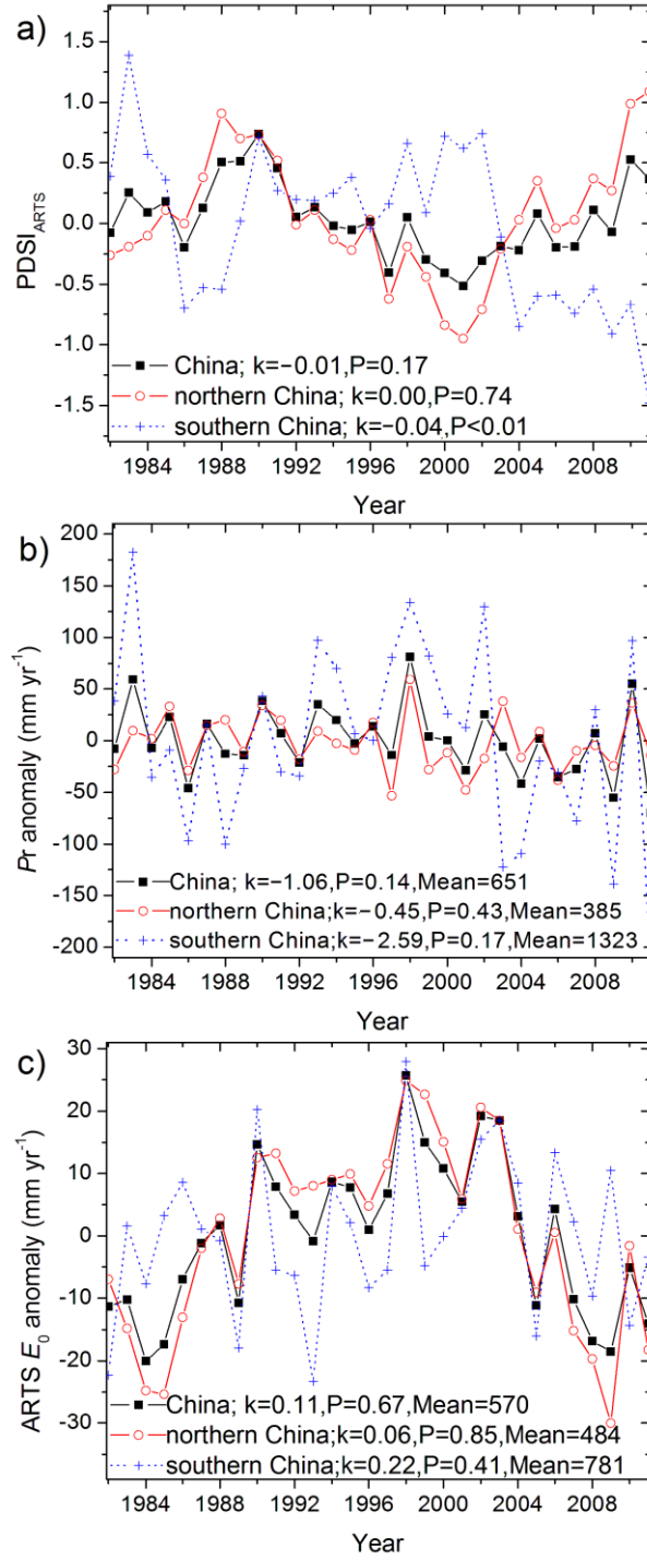
Figure 3. Time series of annual (a) average PDSI_{ARTS} , (b) P_r anomaly, and (c) ARTS E_0 anomaly in whole China, northern China, and southern China during 1982-2011 and slope k and significance P of their linear trends as well as climate mean value.
