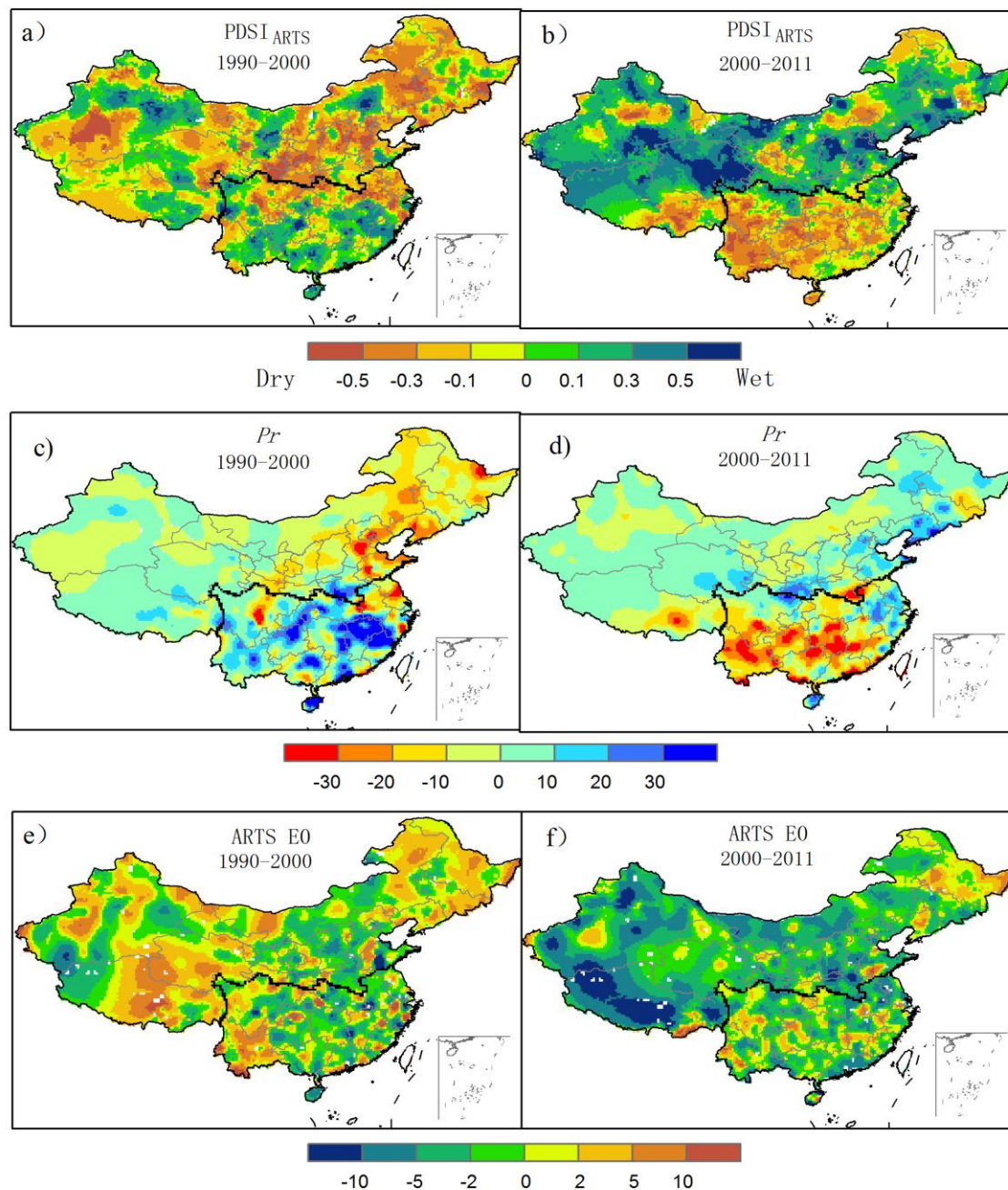
Figure 5. Linear trends of annual (a,b) average PDSI ARTS , (c,d) P_r (mm yr -1 ), and (e,f) ARTS E_0 (mm yr -1 ) during (left) 1990 - 2000 and (right) 2000 - 2011.
