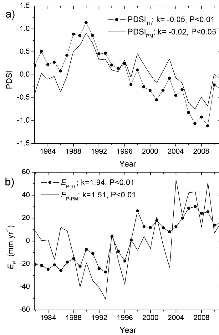
Figure 7. Time series of annual (a) average PDSI_{Th} and PDSI_{PM} , (b) E_{P-Th} and E_{P-PM} for whole China during 1982-2011.
