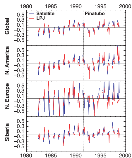
Fig. 1. Monthly boreal zone anomalies of LAI from the AVHRR satellite time series and simulated with the LPJ-DGVM. Due to the low solar angle and snow cover during the winter, only growing season anomalies (May to October) were evaluated. Dotted vertical line indicates time of Pinatubo event.
