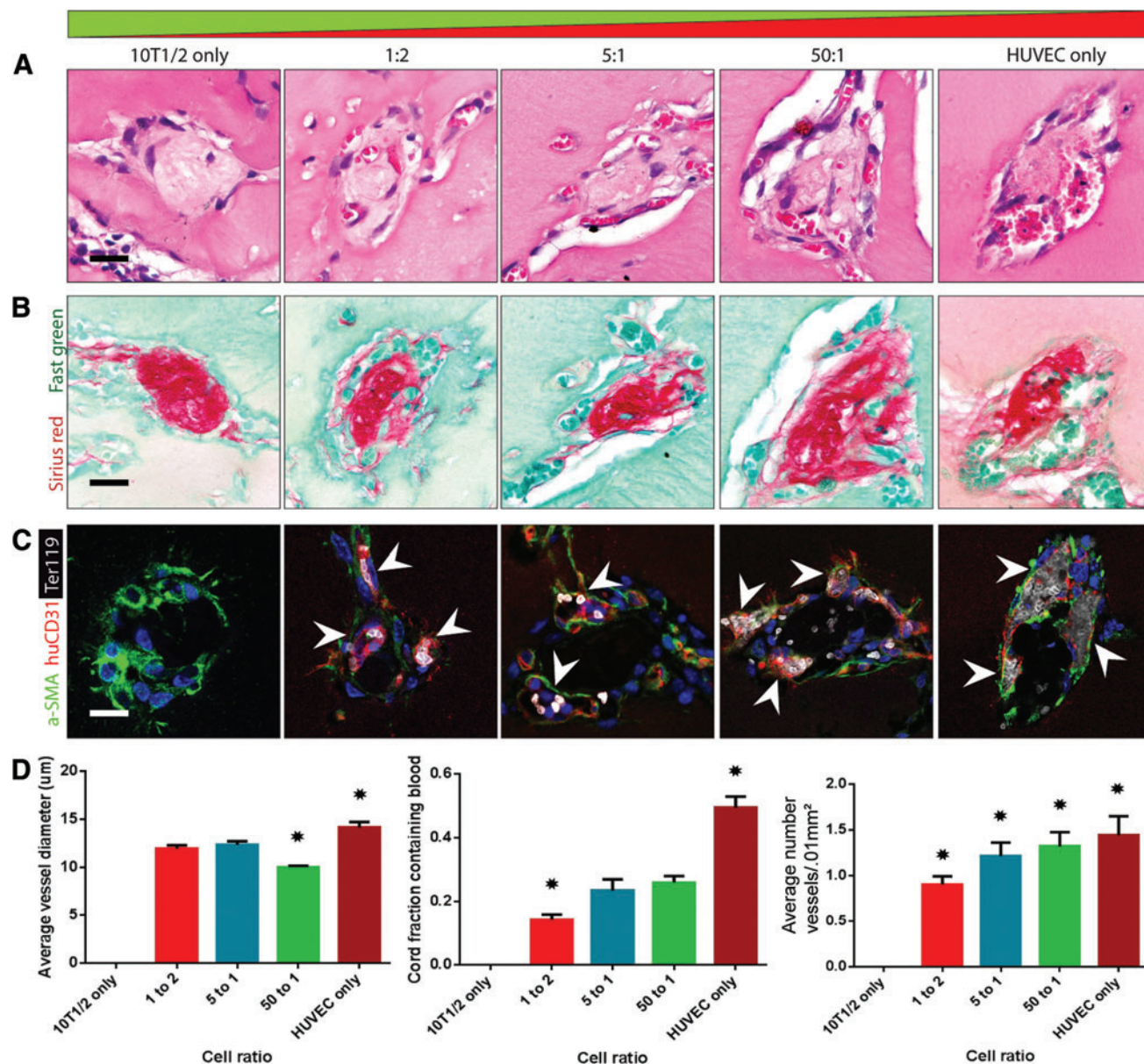
FIG. 3. Endothelial cells in cords are necessary to drive engraftment and integration to host. (A) H&E staining of cords consisting of various EC:10T1/2 ratios (10T1/2 only, 1:2, 5:1, 50:1, HUVEC only) resected after 7 days in vivo suggests the presence of blood in small vessels along the perimeter of all cord conditions containing endothelial cells (scale bar, 50 μm). (B) Sirius red/Fast green staining of collagen within the cords after harvest (scale bar, 50 μm). (C) Ter-119 (erythrocytes, white), human-specific CD31 (HUVECs, red), and alpha-smooth muscle actin (α-SMA; pericytes, green) staining positively identify red blood cells (RBCs) and ECs (arrowheads: individual vessels) and suggest that vessels consist of implanted human endothelium with perivascular colocalization (scale bar, 50 μm). (D) Quantification of blood area, vessel diameter, and vessel numbers for varying cell ratios. *A p-value of <0.05 for comparison. Error bars SEM, n ≥ 20, one-way ANOVA followed by Tukey's post hoc test. HUVEC, human umbilical endothelial cells. Color images available online at www.liebertpub.com/tec
