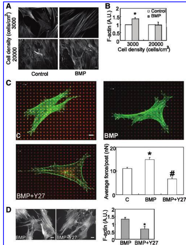
FIG. 3. BMP stimulates cytoskeletal tension. (A) Epifluorescence images of stress fibers in hMSCs plated at 3,000 (upper panels) or 20,000 (lower panels) cells/cm 2 in the absence (left panels, Control) or presence of BMP-2 (right panels, BMP, 100 ng/mL) for 1 h. (B) Quantification results of stress fiber formation in hMSCs plated at 3,000 or 20,000 cells/cm 2 in the absence or presence of BMP-2 (100 ng/mL) (* P < 0.05 vs. paired control). A.U. represents arbitrary unit. (C) Representative images of control (C), BMP-2 (100 ng/mL) (BMP) and BMP-2 plus Y27632 (25 μM) (BMP + Y27) treated hMSC on mPAD (red, mPAD; green, actin cytoskeleton; blue, nuclei). Plot of average traction force exerted on each underlying post were presented as mean ± SEM of 3 independent experiments (* P < 0.01 vs. C; # P < 0.01 between BMP-2 and BMP-2 + Y27). Scale bar: 20 μm. (D) Fluorescence images and quantification plot of stress fibers in hMSCs plated at 3,000 cells/cm 2 and treated with Y27632 (10 μM) in the presence of BMP-2 (100 ng/mL) for 1 h. mPAD, microfabricated postarray detector. Color images available online at www.liebertonline.com/scd
