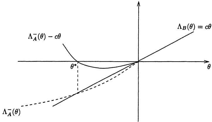
FIG. 8. Notice that at \theta^* we have \Lambda_A^{-\prime}(\theta^*) \leq c . Thus, when a \geq c , the optimizer \hat{\theta} satisfies 0 \geq \hat{\theta} \geq \theta^* , which implies \Lambda_{\Gamma}^{*-}(a) = \Lambda_A^{*-}(a) .
