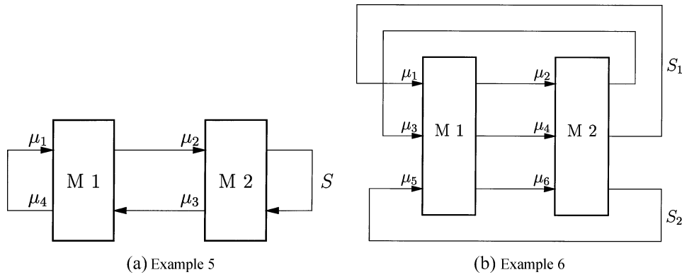
Fig. 6. Exponential service times with rate \mu_i for class i . (a) Example 5: Total number of jobs equals S , \mathbf{h} = \mathbf{e}/4 , \boldsymbol{\mu} = (1/3, 2/7, 1, 2) . (b) Example 6: Type 1 jobs (classes 1–4) are fixed to S_1 , type 2 jobs (classes 5–6) are fixed to S_2 , \mathbf{h} = (1/4, 1/4, 1/4, 1/4, 1/2, 1/2) , \boldsymbol{\mu} = (8, 5, 2, 7, 4, 1) .
