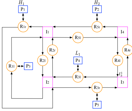
Fig. 2. Transition system \mathcal{T}_1 for robot 1 in RULE (Fig. 1). The output h_1 captures the locations of the unsafe regions and the requests. The dummy request \varpi_1 and the initial state are omitted in this figure.
