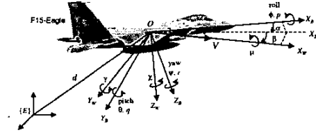
Figure 1: Body reference frames on an aircraft.
