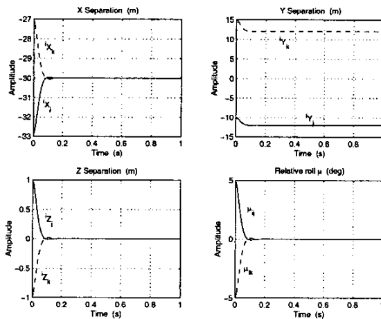
Figure 4: Controlled output variables of follower UAVs.
