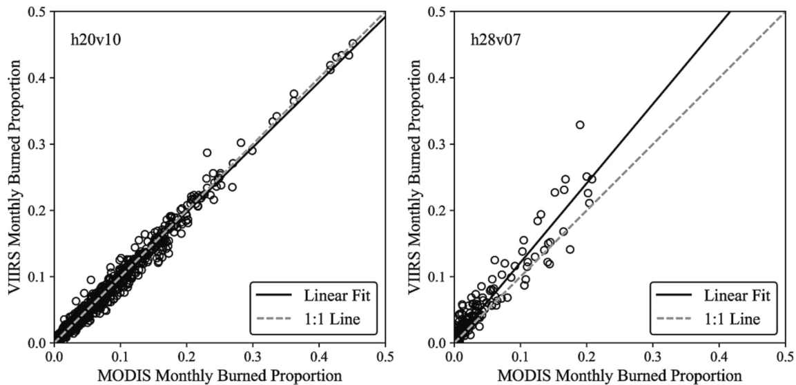
Fig. 35. Scatter plots of the monthly proportions of coarse resolution \sim 120 \times 120 km cells labeled as burned in the Collection 2 VIIRS VNP64A1 burned area product, plotted against the corresponding proportion labeled as burned in the Collection 6.1 MODIS burned area product over a 31-month test period (July 2018 – Feb. 2020 + Feb. 2021 – Dec. 2021). Plots are for MODIS tiles located in southern Africa (h20v10; left panel) and southeast Asia (h28v07; right panel) and are representative of product consistency in savanna/non-agricultural (Pearson’s r = 0.994 ) and agricultural ( r = 0.963 ) regions, respectively. Solid black lines show the ordinary least squares regression lines; dashed gray 1-to-1 lines are included for reference.
