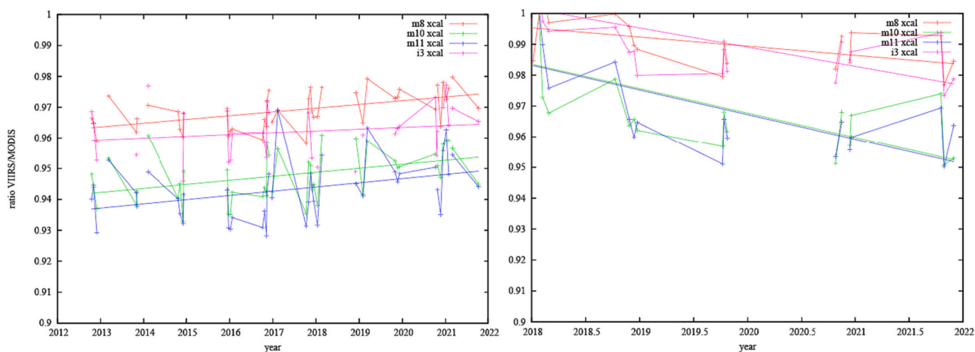
Fig. 6. Intercalibration ratios derived over Sun Glint for the VIIRS SWIR bands, SNPP (left), NOAA-20 (right).
