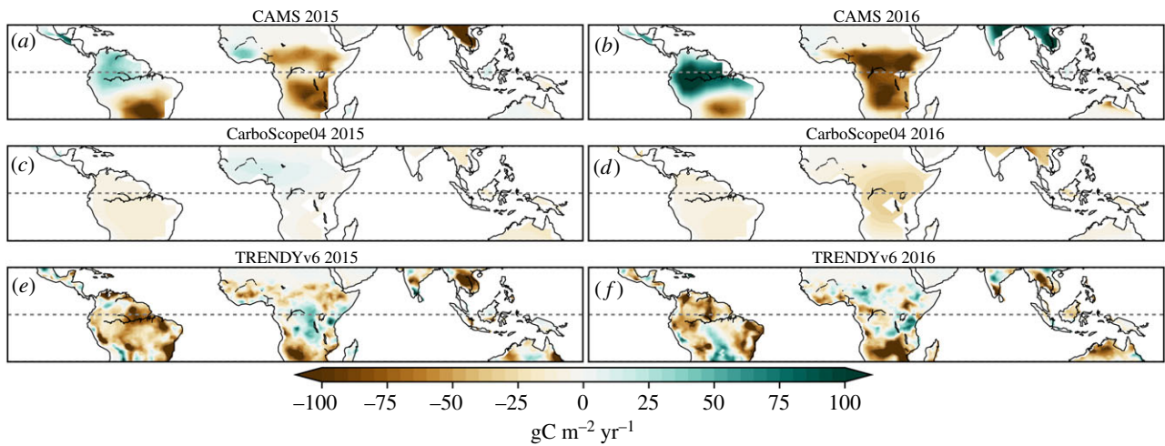
Figure 2. \text{NBP}_{\text{anom}} maps for the two recent El Niño years (2015/2016, (a,c,e)/(b,d,f)) estimated by CAMS (a,b) and CarboScope04 (c,d) inversions and the TRENDYv6 MMEM (e,f). Anomalies are calculated by deseasonalising and detrending the time-series for each pixel for 1979–2016 (2004–2016 for CarboScope04). Positive anomalies correspond to a stronger-than-average \text{CO}_2 sink or a below-average source.
