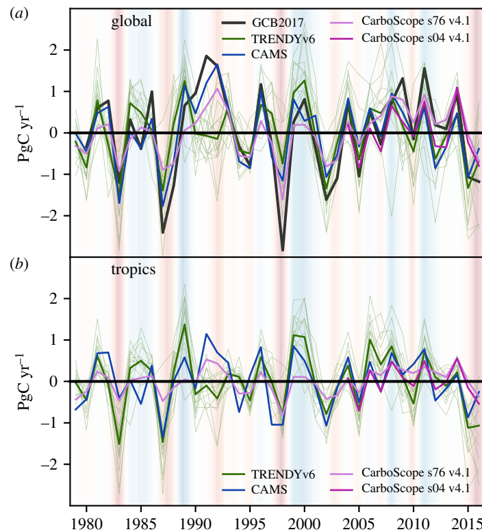
Figure 1. Time-series of detrended annual \text{NBP}_{\text{anom}} for the globe (a) and tropical regions (b), estimated as the residual sink by GCB2017 (black, globe only), CAMS v16r1 (blue), CarboScope76 (light magenta) and CarboScope04 (magenta) atmospheric inversions and TRENDYv6 models (green, thicker line indicates the multi-model ensemble mean (MMEM)). \text{NBP}_{\text{anom}} is defined as the net atmosphere-to-land \text{CO}_2 flux: positive anomalies indicate stronger-than-average \text{CO}_2 sinks or lower-than-average \text{CO}_2 sources. The shades in the background of both panels show the ENSO states (red – El Niño and blue – La Niña).
