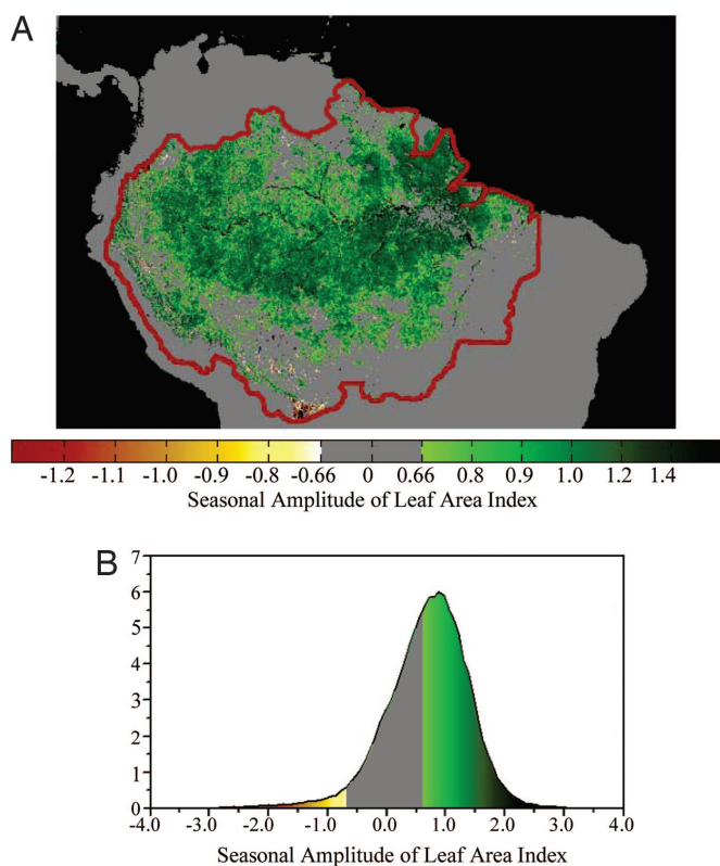
Fig. 2. Seasonal amplitude of LAI. (A) Color-coded map of LAI amplitudes greater than 0.66 or less than -0.66 ; this threshold (0.66) is the smallest LAI difference discernable with the MODIS LAI data set (see SI Materials and Methods). In regions with dry seasons longer than 3 months, the amplitude is calculated as the difference between the maximum 4-month average LAI in the dry season minus the minimum 4-month average LAI in the wet season. Where the dry season is three or fewer months, the amplitude is calculated as the difference between the dry-season average LAI and the minimum 4-month average LAI in the wet season. The dry and wet seasons are defined based on the precipitation data set at 15' spatial resolution (see SI Materials and Methods). Thus, the seasons vary spatially and interannually. (B) Distribution of LAI amplitude for all Amazon rainforest pixels. The color scheme is similar to that in A.
